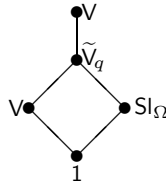
FIGURE 2. \mathcal{L}_Q(\tilde{\mathbf{V}})
