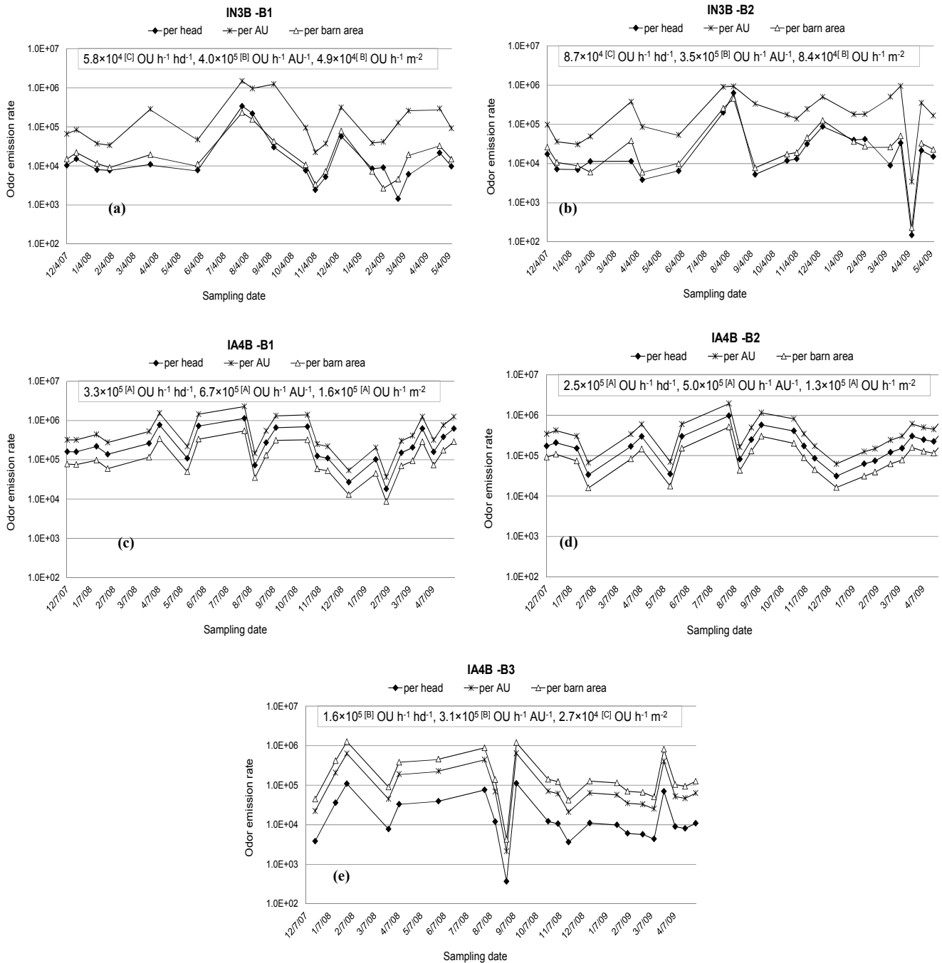
Figure 5. Average barn odor emission rates of sites IN3B (swine finishing) and IA4B (barns 1 and 2 were swine gestation barns, and barn 3 was a swine farrowing barn). Averages of three measurements are reported for IN3B and two measurements for IA4B for each sampling day (total of 25 sampling days per site). Overall average emission rate values (shown in boxes) followed by different letters are significantly different ( p < 0.05 ). Emission rates in \text{OU h}^{-1} \text{m}^{-2} , \text{OU h}^{-1} \text{hd}^{-1} , and \text{OU h}^{-1} \text{AU}^{-1} were evaluated separately. The y-axis is a log scale.
