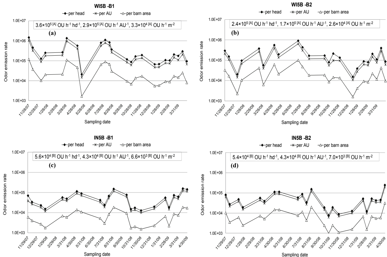
Figure 4. Average barn odor emission rates at freestall dairy sites W15B and IN5B. Averages of three measurements are reported for each sampling day (total of 25 sampling days per site). Overall average emission rate values (shown in boxes) followed by different letters are significantly different ( p < 0.05 ). Emission rates in \text{OU h}^{-1} \text{m}^{-2} , \text{OU h}^{-1} \text{head}^{-1} , and \text{OU h}^{-1} \text{AU}^{-1} were evaluated separately. The y-axis is a log scale.
