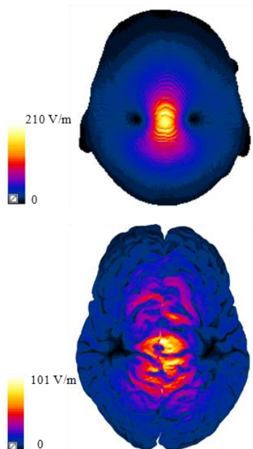
Fig. 4. Induced electric field in skin (top) and grey matter (bottom) from one of the head models.
