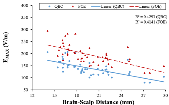
Fig. 6. Comparison between the maximum induced electric field ( E_{MAX} ) versus brain-scalp distance for 50 head models, using the Quadruple Butterfly Coil and Figure-of-Eight Coil.
