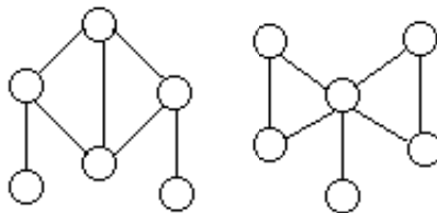
FIG. 1.2. Cospectral graphs with p(x) = -1 + 4x + 7x^2 - 4x^3 - 7x^4 + x^6 .
