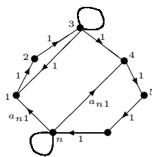
FIG. 3.1. Nonzero- L -digraph of the completion of A for Case 3D
