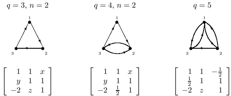
FIG. 4.1. Digraphs that do not have completion
