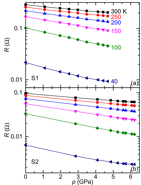
FIG. 2. Pressure dependence of resistance R(p) at fixed temperatures for \text{EuRbFe}_4\text{As}_4 sample 1 (a) and sample 2 (b).
