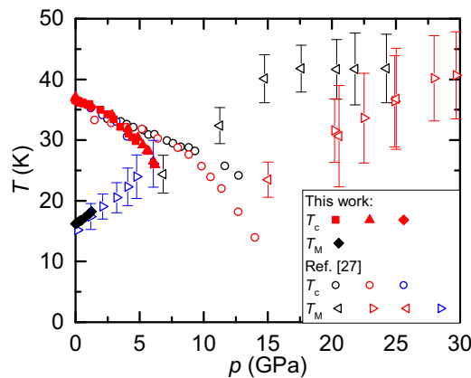
FIG. 7. Pressure-temperature phase diagram of \text{EuRbFe}_4\text{As}_4 up to \sim 30 GPa, including data from Ref. [27] (open symbols). Open circles corresponds to the onset of the superconducting transition measured via resistivity or magnetic susceptibility. Open triangles corresponds to the magnetic transition determined from magnetic susceptibility or feature in d\rho/dT .
