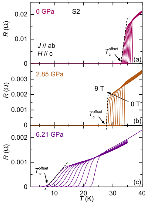
FIG. 3. Temperature dependence of resistance under magnetic field up to 9 T for selective pressures for sample 2. Criteria for T_c^{\text{offset}} under magnetic fields are indicated by arrows. Current was applied in-plane and magnetic field was applied along the c axis.
