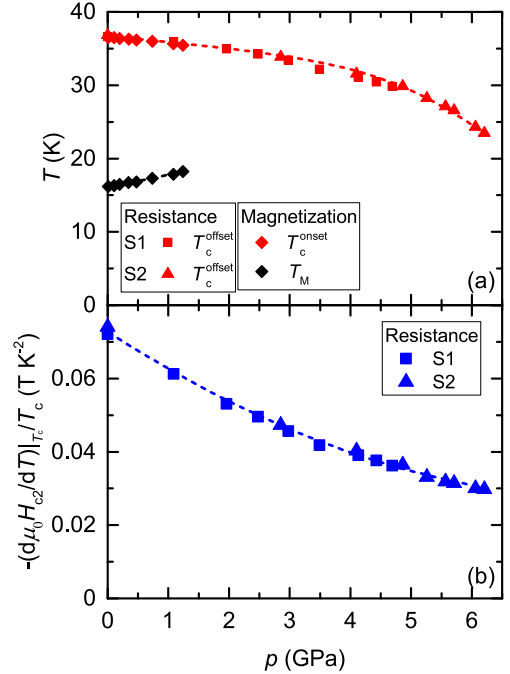
FIG. 6. (a) Pressure-temperature phase diagram of \text{EuRbFe}_4\text{As}_4 , as determined from resistance and magnetization measurements. Red and black symbols represent the superconducting T_c^{\text{offset}} and magnetic T_M phase transitions. (b) Pressure dependence of the normalized upper critical field slope -(1/T_c)(d\mu_0 H_{c2}/dT)|_{T_c} . The squares and triangles are data obtained from resistance measurement for sample 1 and sample 2, respectively. The diamonds are data obtained from magnetization measurement. Dashed lines are guides to the eye.
