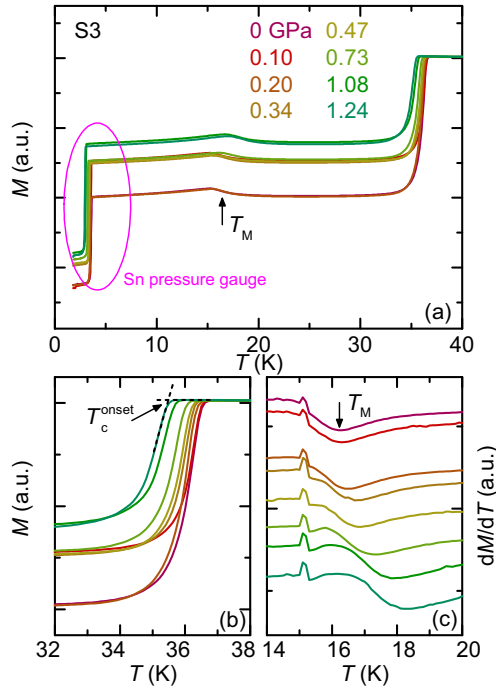
FIG. 5. (a) Evolution of the zero-field-cooled (ZFC) magnetization M(T) with hydrostatic pressures up to 1.24 GPa under 20 mT applied field. Superconducting transition of Sn is used to determine the low temperature pressure, as indicated by the pink circle. (b) Blowup of the superconducting transition region for \text{EuRbFe}_4\text{As}_4 . The criterion for T_c^{\text{onset}} is indicated by an arrow. (c) Temperature derivative of the magnetization, dM/dT , showing the evolution of the magnetic transition T_M . The criterion is indicated by an arrow. The small feature just above 15 K is an artifact caused by the combination of small temperature steps and details of the temperature control in MPMS-3.
