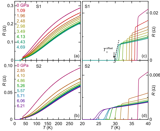
FIG. 1. (a),(b) Evolution of the in-plane resistance with hydrostatic pressures up to 6.21 GPa measured in a mBAC for \text{EuRbFe}_4\text{As}_4 sample 1 and sample 2, respectively. (c),(d) Blowups of the low temperature region showing the superconducting transition. The criterion for T_c^{\text{offset}} is indicated by an arrow in (c).
