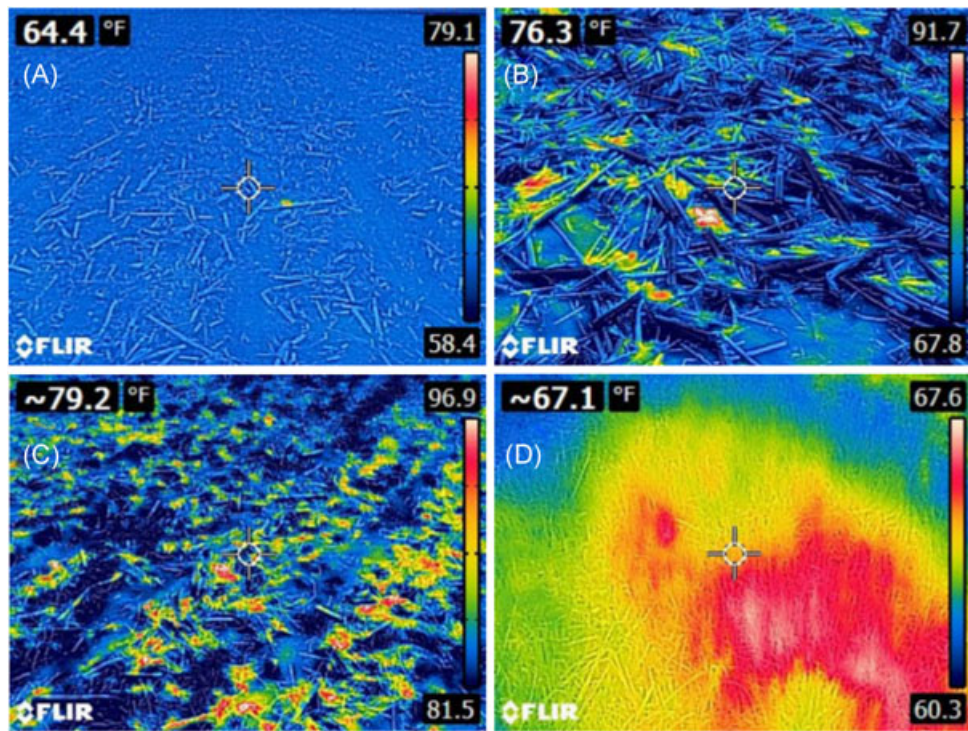
Figure 1. Example views through a thermal imager used to detect avian nests in Iowa, USA, during 2016. The temperature in the upper left is a measurement of the thermal energy being emitted or reflected from the object in the crosshairs, not the ambient air temperature. The red–blue scale on the right of each image shows the range of emissivity values represented within the field of view. (A) Vesper sparrow nest (just right of cross hairs) in a barren agricultural field before dawn. (B) Killdeer nest (just below and to the left of cross hairs) in a barren agricultural field within an hour after dawn. (C) Direct sunlight early in the morning reflects off many surfaces, creating a confusing image. There is no nest in this view. (D) Smooth brome grass monoculture with strong reflected solar rays in the early afternoon. There is no nest in this view.
