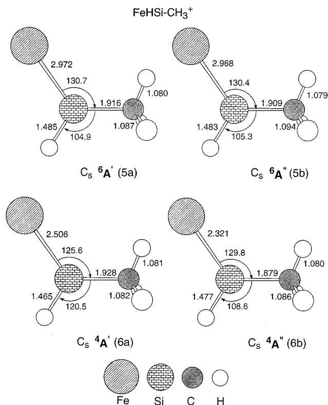
Figure 4. CASSCF (11/10) optimized geometries of the FeHSi-CH 3 + methyl structure isomer of FeSiCH 4 + for the low-lying electronic states (bond lengths in Å, bond angles in deg).
