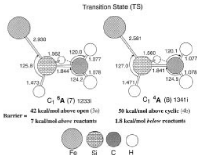
Figure 5. CASSCF (11/10) optimized geometries of the transition states for the interconversion between the open H 2 Si-CH 2 Fe + 6 A' ( 3a ) and methyl structure FeHSi-CH 3 + 6 A'' ( 5b ) and between cyclic (H 2 Si-CH 2 )Fe + 4 A'' ( 4b ) and methyl structure FeHSi-CH 3 + 4 A'' ( 6b ) (bond lengths in Å, bond angles in deg).
