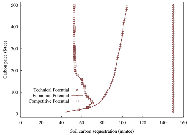
PANEL A Mitigation potentials of soil carbon sequestration on U.S. cropland including conversion of cropland into pastureland
