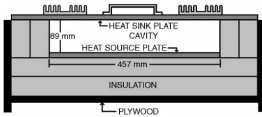
Fig. 1. Cross-section of laboratory heat flow chamber.
