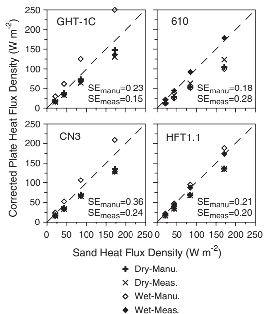
Fig. 2. Corrected plate heat flux density ( G_m ) for four plate designs vs. known heat flux density ( G ) in dry and saturated quartz sand using manufacturer-specified and measured plate dimensions and thermal conductivities ( \lambda_m ). Original flux plate data taken from Sauer et al. (2003).
