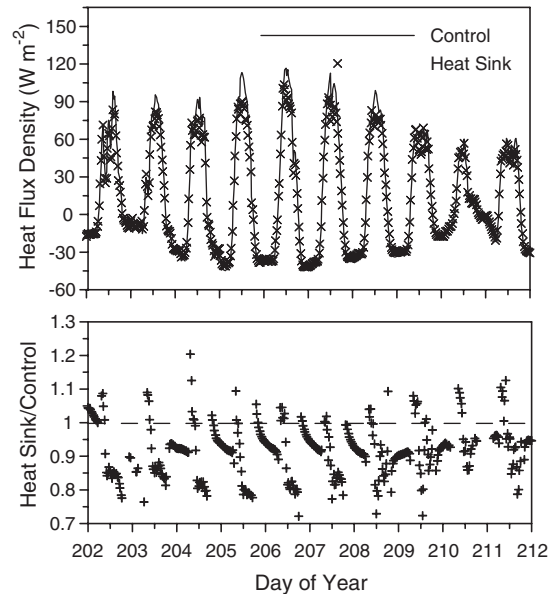
Fig. 4. (Top) mean heat flux density of triplicate control and heat sink compound-coated flux plates in Waukegan silt loam and (bottom) the ratio of plate heat flux density ( G_m ) for plates with and without Arctic Silver 5 heat sink compound.
