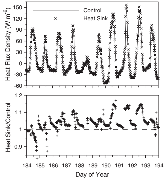
Fig. 3. (Top) mean heat flux density of triplicate control and heat sink compound-coated flux plates in Waukegan silt loam and (bottom) the ratio of plate heat flux density ( G_m ) for plates with and without water-soluble heat sink compound.
