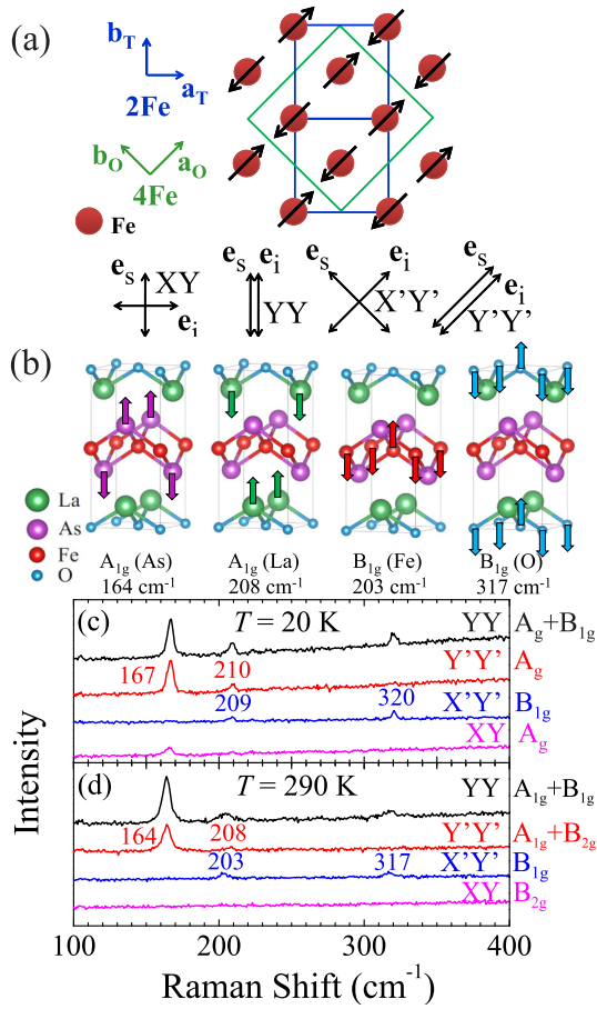
FIG. 1. (a) Schematic view of the Fe square lattice with the stripe antiferromagnetic structure and representations of the XY , YY , X'Y' , and Y'Y' linear polarizations. The unit vectors e_i and e_s represent the polarizations of the incident and scattered photons, respectively. The edges and axes for the 2 Fe tetragonal and 4 Fe orthorhombic unit cells are also displayed. (b) Raman-active phonons accessible in the scattering geometry employed in this paper. The corresponding symmetries and observed frequencies at 290 K are indicated. (c,d) Raman spectra for distinct polarizations at T = 20 K (c) and T = 290 K (d). In (c) and (d), the symmetry associated with each polarization is given with respect to the corresponding orthorhombic and tetragonal unit cells.
