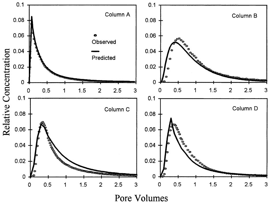
Fig. 2. Observed and calculated effluent BTC. Calculated BTC were obtained using TDR-determined mobile/immobile model parameters and the CXTFIT program.
