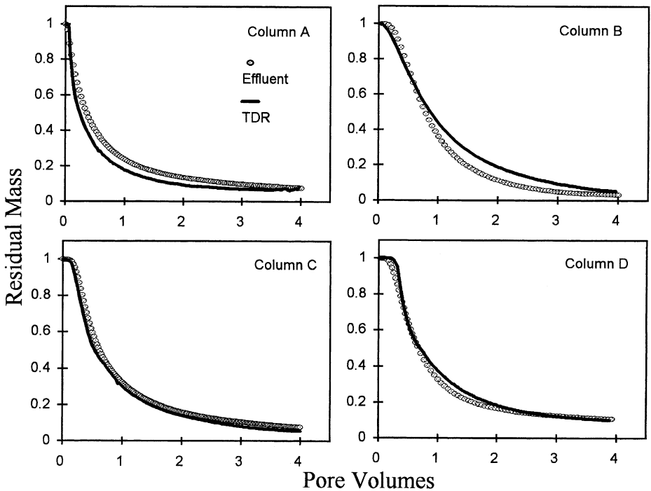
Fig. 1. Residual mass breakthrough curves (BTC) obtained from TDR and from effluent data.
