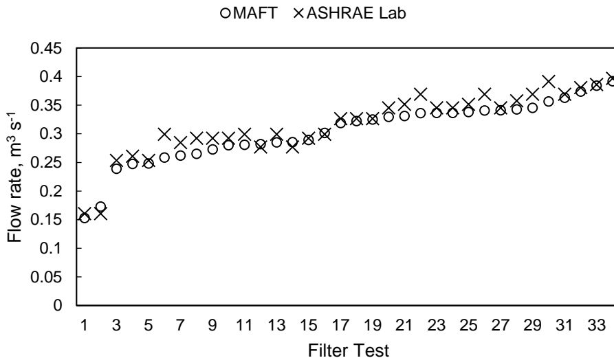
Figure 2. MAFT flowrates and ASHRAE 52.2 certified lab flowrates for validation filter tests.
