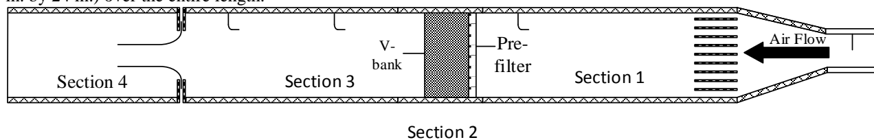
Figure 1. MAFT duct sections as assembled.
