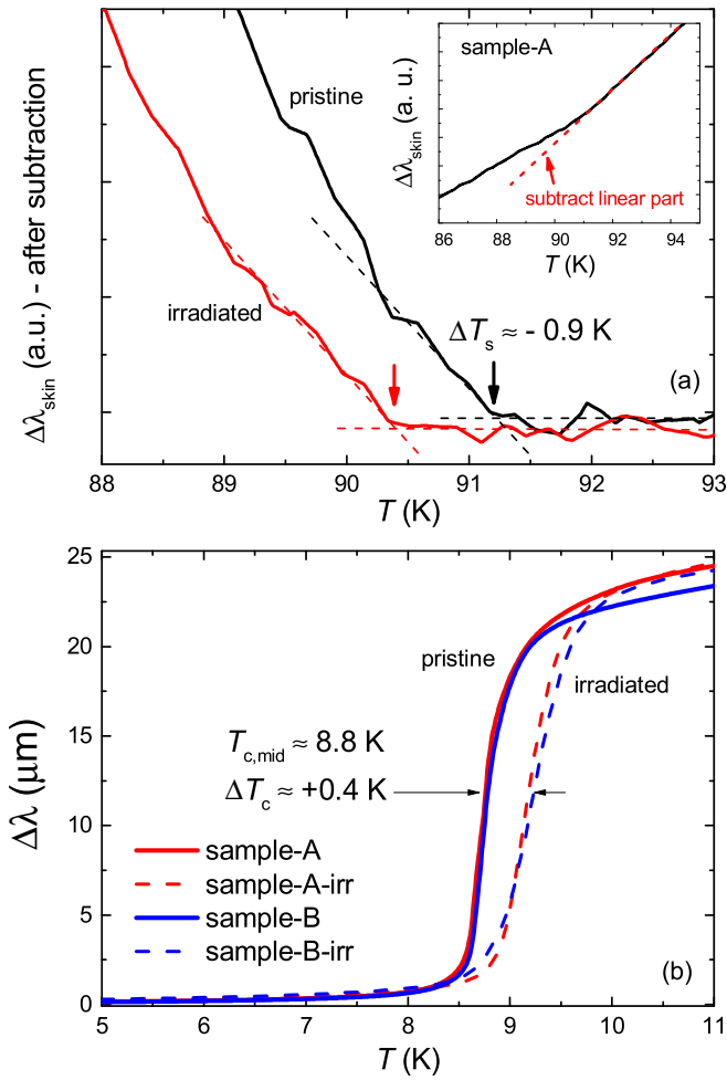
FIG. 1. (a) Variation of normal state skin depth \Delta\lambda_{\text{skin}}(T \gg T_c) of sample A after linear subtraction as shown in the inset. Arrows mark structural transition T_s before and after 2.5 MeV electron irradiation of 1.8 C/cm 2 . (b) London penetration depth \Delta\lambda(T) before and after electron irradiation in samples A and B.
