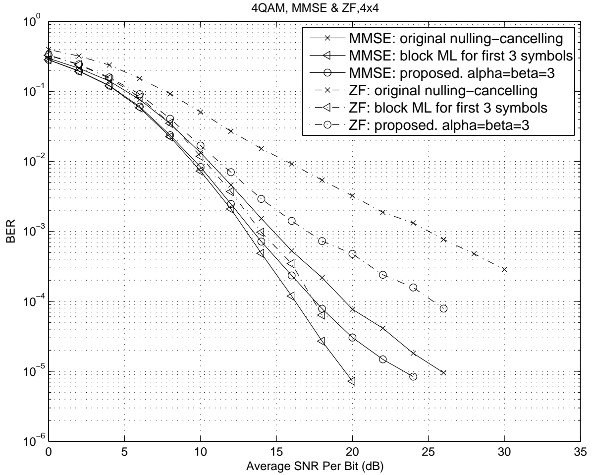
Figure 5.5 BER of decoding algorithms versus E_b/N_0 per transmit antenna, M = N = 4 ; 4-QAM, MMSE & ZF
