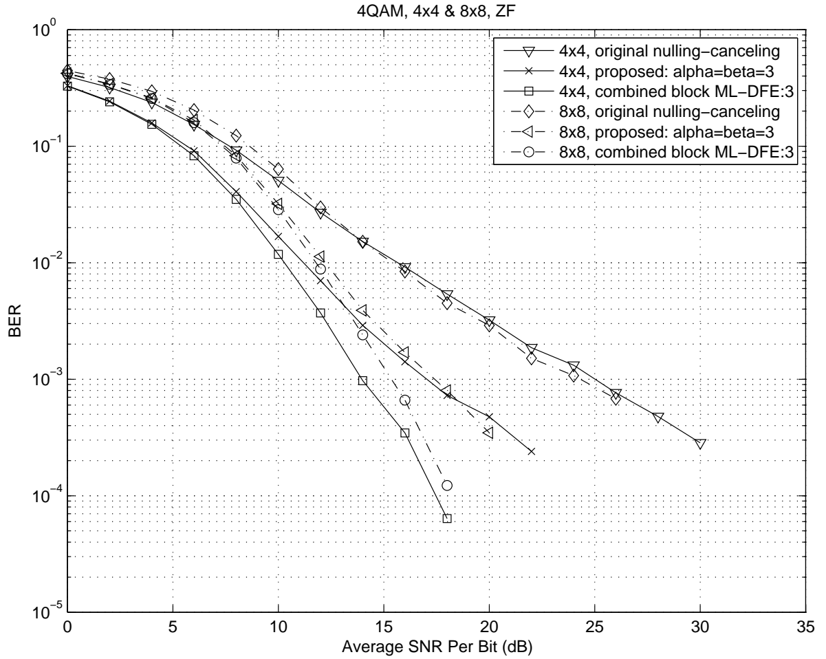
Figure 5.7 BER of decoding algorithms versus E_b/N_0 per transmit antenna, M = N = 4 or M = N = 8 ; 4-QAM, ZF
