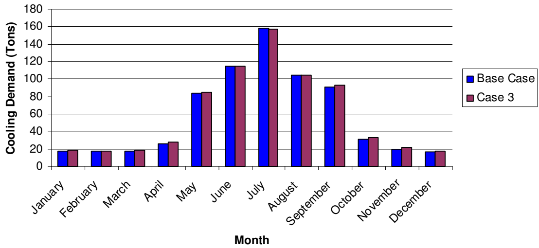
Figure 4.8 Average Monthly Cooling Demand for Case 3 and the Base Case
