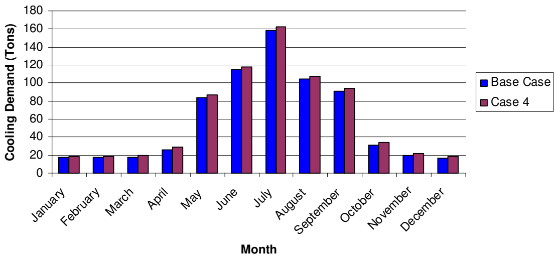
Figure 4.10 Average Monthly Cooling Demand for Case 4 and the Base Case
