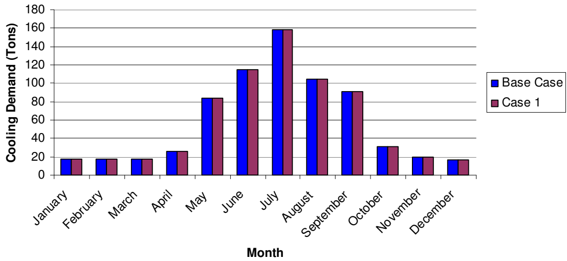
Figure 4.2 Average Monthly Cooling Demand for Case 1 and the Base Case
