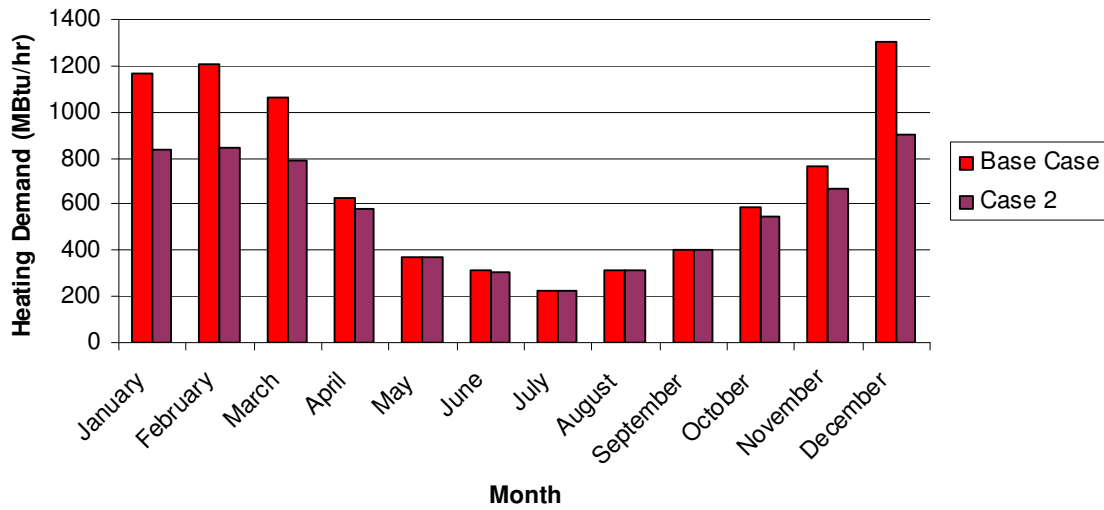
Figure 4.5 Average Monthly Heating Demand for Case 2 and the Base Case
