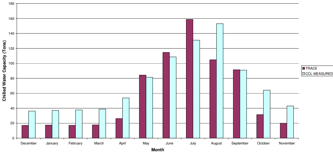
Figure 3.5 Predicted versus actual Chilled Water Usage
