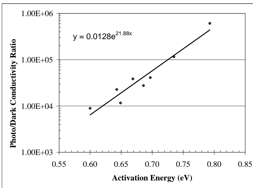
Figure 4.3 Photo/Dark conductivity ratios plotted versus activation energy.
