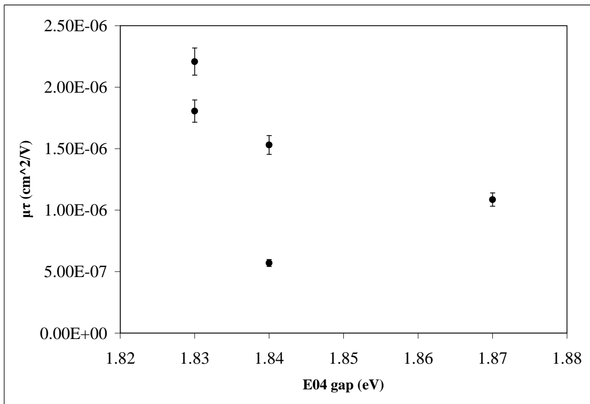
Figure 4.13 Electron \mu\tau_{eff} versus E04 gap.
