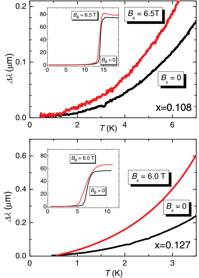
FIG. 8. (Color online) Effect of heavy-ion irradiation on London penetration depth, \Delta\lambda(T) in samples with x = 0.108 (top) and x = 0.127 (bottom). Black curves show pristine samples, red curves show irradiated with matching fields of 6.5 T and 6 T, respectively. Insets show the variation of the London penetration depth in the entire range to T_c .
