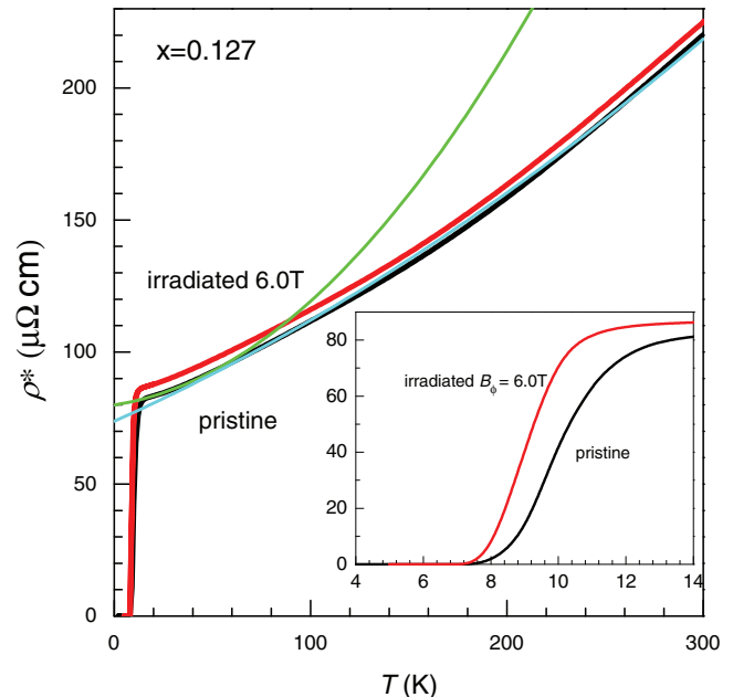
FIG. 2. (Color online) Comparison of the temperature-dependent electrical resistivity of reference and irradiated samples x = 0.127 , with a geometric factor correction by normalizing slopes of the \rho(T) curves at 300 K. For the pristine sample, we assumed \rho(300\text{K}) = 220\ \mu\Omega\text{cm} . 49 Inset zooms for the superconducting transition range. Heavy ion irradiation does not change the shape of the \rho(T) curves, but increases residual resistivity, sharpens the superconducting transition, and shifts T_c downward.
