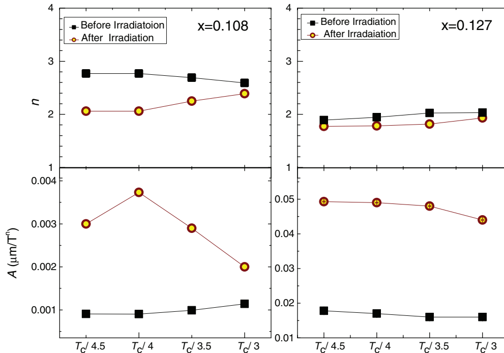
FIG. 9. (Color online) Dependence of the fitting parameters, n (top panels) and A (bottom panels), of the power-law function, \Delta\lambda = AT^n , on the temperature of the high-temperature boundary of the fitting interval. Data are shown for pristine (black squares) and irradiated (yellow-brown circles) sample with x = 0.108 (left) and x = 0.127 (right).
