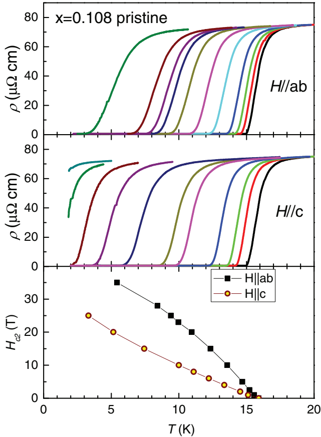
FIG. 3. (Color online) In-plane resistivity \rho(T) for slightly overdoped \text{Ba}(\text{Fe}_{1-x}\text{Co}_x)_2\text{As}_2 , x = 0.108 , in magnetic fields (a) parallel to the conducting plane, perpendicular to the c axis, and (b) parallel to the crystallographic c axis. The field values are (right to left) 0, 1, 2.5, 5, 10, 15, 20, 23, 25, 28, and 35 T. The bottom panel (c) shows H_{c2}(T) phase diagrams for both directions of the magnetic field.
