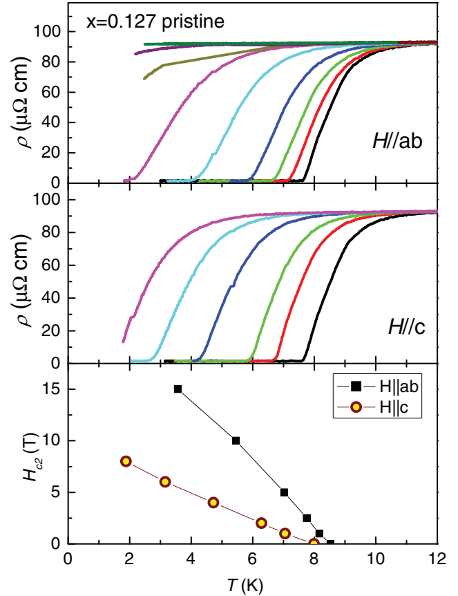
FIG. 4. (Color online) In-plane resistivity \rho(T) for heavily overdoped \text{Ba}(\text{Fe}_{1-x}\text{Co}_x)_2\text{As}_2 , x = 0.127 in magnetic fields (a) parallel to the conducting plane and perpendicular to the c axis, field values (right to left) 0, 1, 2.5, 5, 10, 15, 20, 23, and 25 T, and (b) parallel to the crystallographic c axis, field values (right to left) 0, 1, 2, 4, 6, 8, and 10 T. Bottom panel (c) shows H_{c2}(T) phase diagrams for both directions of magnetic field.
