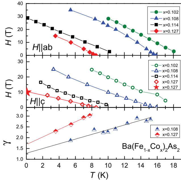
FIG. 5. (Color online) H_{c2}(T) and anisotropy parameter, \gamma \equiv H_{c2,ab}/H_{c2,c} , for overdoped samples of BaCo122 x = 0.108 and x = 0.127 . Top panel shows configurations with magnetic fields parallel to the conducting plane. The middle panel shows configurations with the magnetic field parallel to the crystallographic c axis. For reference, we show bulk H_{c2,c}(0) as determined from the thermal conductivity study in the sample x = 0.127 (red star, Ref. 18), which suggests the data for strongly overdoped samples x = 0.127 show very close to T -linear dependence. The top and middle panels show data for previously studied overdoped samples with x = 0.102 and x = 0.114 , 41 determined using the same midpoint criterion. The bottom panel shows the temperature-dependent anisotropy parameter for samples x = 0.108 and x = 0.127 .
