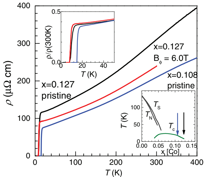
FIG. 1. (Color online) Temperature-dependent electrical resistivity for the reference samples x = 0.108 and x = 0.127 , and the irradiated sample of x = 0.127 . The irradiated sample x = 0.127 is the same sample as used in penetration depth measurements, with contacts soldered after measurements completed. The top inset shows the same curves using a normalized resistivity scale \rho/\rho(300\text{K}) , showing the main difference between resistivity values comes from the error of geometric factor determination. 41,47 The bottom inset shows a sketch of the doping phase diagram for BaCo122 with the position of the samples used in this study.
