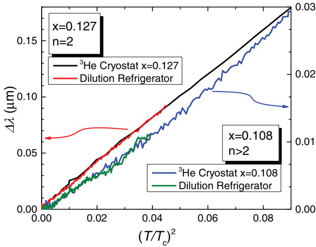
FIG. 7. (Color online) Low temperature London penetration depth \Delta\lambda(T) measured in single crystals of \text{Ba}(\text{Fe}_{1-x}\text{Co}_x)_2\text{As}_2 with x = 0.108 (green and blue curves) and x = 0.127 (black and red curves) plotted vs (T/T_c)^2 . Linear plot for x = 0.127 shows the dependence is very close to T^2 , consistent with more detailed fitting analysis using a floating fitting range, see Fig. 9. Clear deviations for sample x = 0.108 suggest n > 2 .
