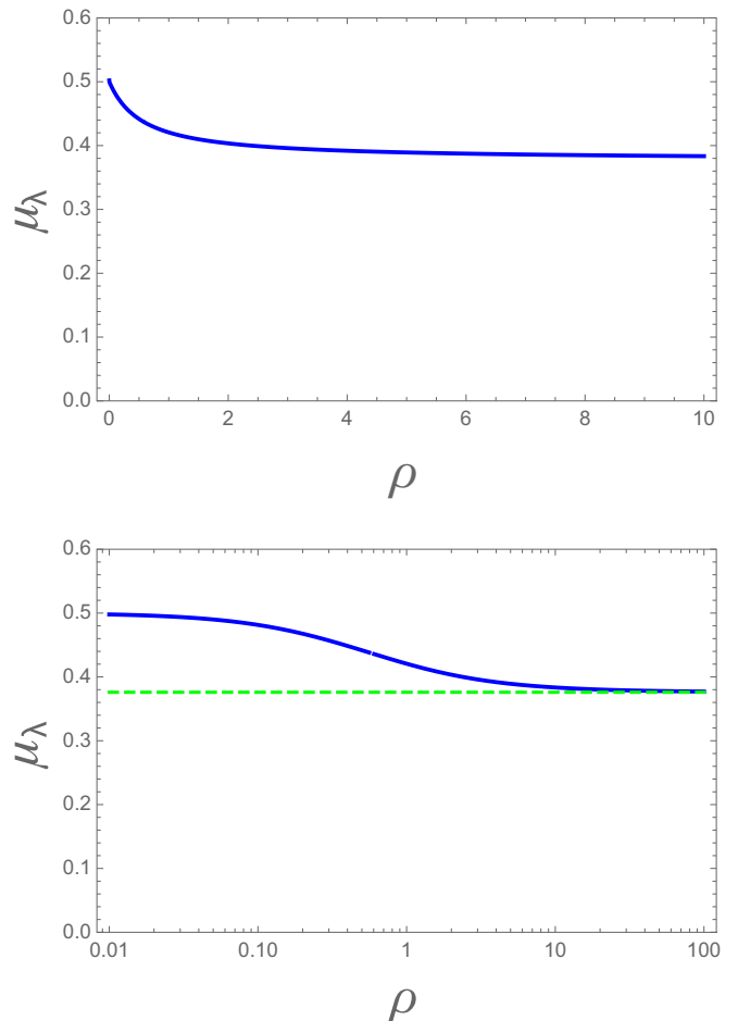
FIG. 1. Top panel: \mu_\lambda vs \rho . Lower panel: the same on a semilog scale; the dashed line is the dirty limit value.
