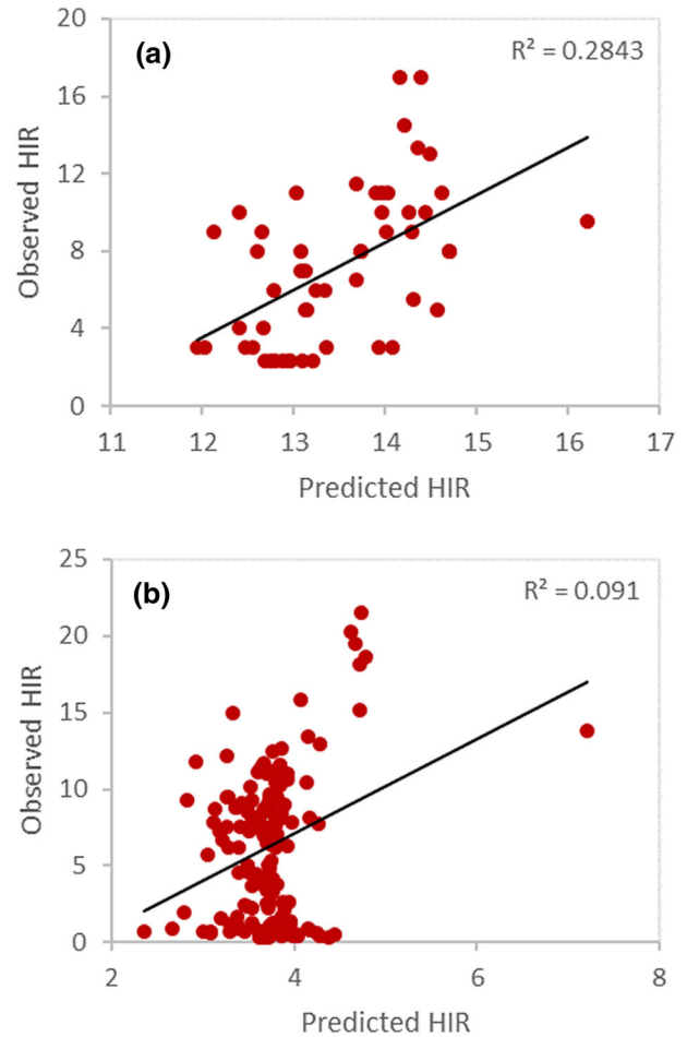
FIGURE 2 Linear regression of the 53 inducers genomic estimated breeding values with their observed values, using the ISU inducer set as training population (a). Linear regression of the 159 inducers genomic estimated breeding values with their observed values, using the UOH inducer set as training population (b)
