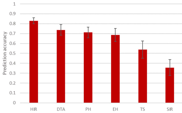
FIGURE 1 Average cross-validation prediction accuracies and standard deviation observed in the ISU inducer set, for the following traits: haploid induction rate (HIR, %); days to anthesis (DTA, GDUs); plant height (PH, cm); ear height (EH, cm); tassel size (TS, cm); self-induction rate (SIR, %)
