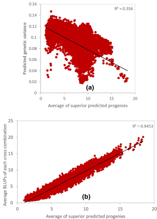
FIGURE 3 Relationship between the average of superior predicted progenies ( \mu_{SP} ) and predicted genetic variance ( V_G ) (a) and average BLUPs of each possible crossing combination (b) for HIR (%) in each of the 12,561 predicted crosses
