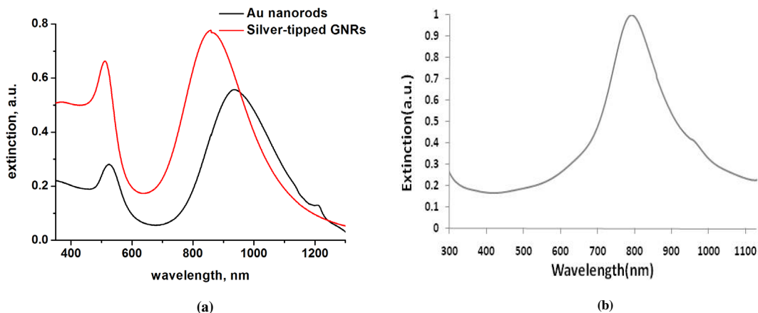
Figure 3. Surface plasmon characteristics of (a) gold nanorods and silver-tipped gold nanorods and (b) Au-Ag alloy nanocages.
