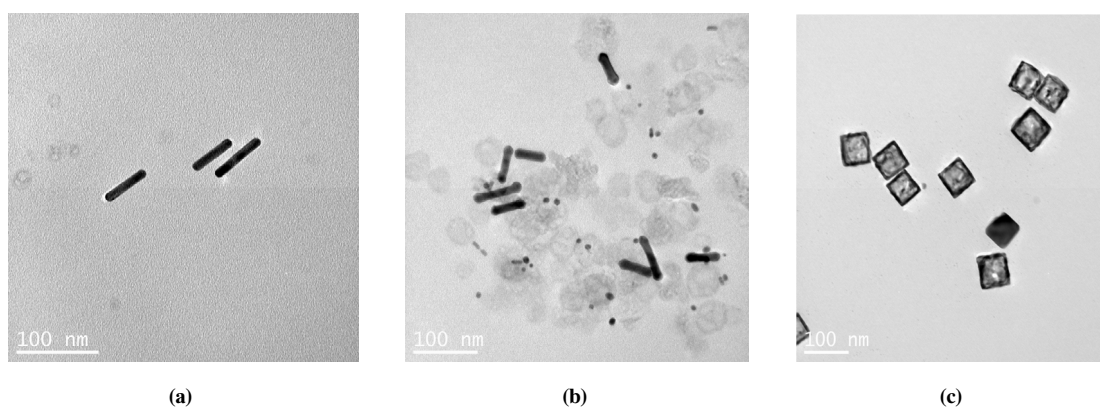
Figure 1. TEM images of (a) gold nanorods, (b) silver-tipped gold nanorods, and (c) Au-Ag alloy nanocages.
