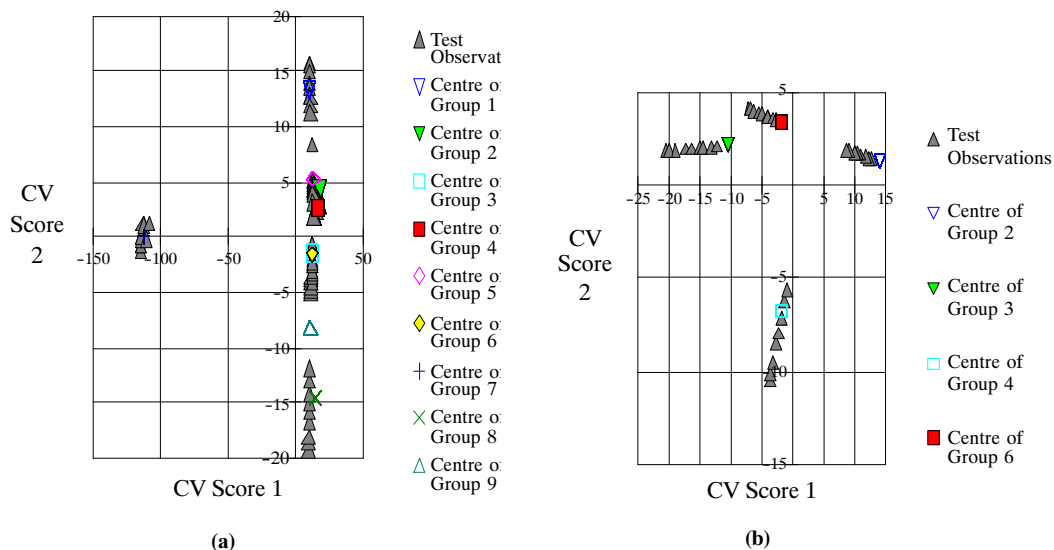
Figure 7. CVA analysis of sm2 (table 6): (a) first round and (b) second round.
