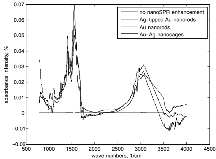
Figure 2. nanoSPR enhanced IR spectrum of E. coli O103 at 10^3 CFU mL -1 .
