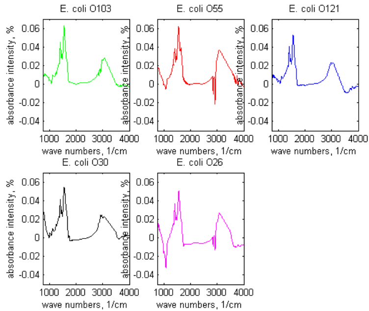
Figure 4. Spectra of the five E. coli strains under nanoSPR enhancement of Au-Ag alloy nanocages.
