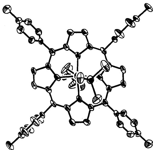
Figure 4. ORTEP drawing of trans -(TTP)Os=CH-SiMe 3 (THF): axial view showing the relationship between the (trimethylsilyl)methylidene fragment and the porphyrin ring.
