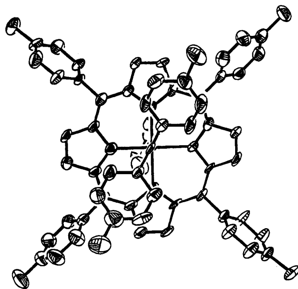
Figure 2. ORTEP drawing of trans -(TTP)Os=C(C 6 H 4 - p -CH 3 ) 2 (THF): axial view showing the relationship between the di-p -tolylmethylidene fragment and the porphyrin ring.
