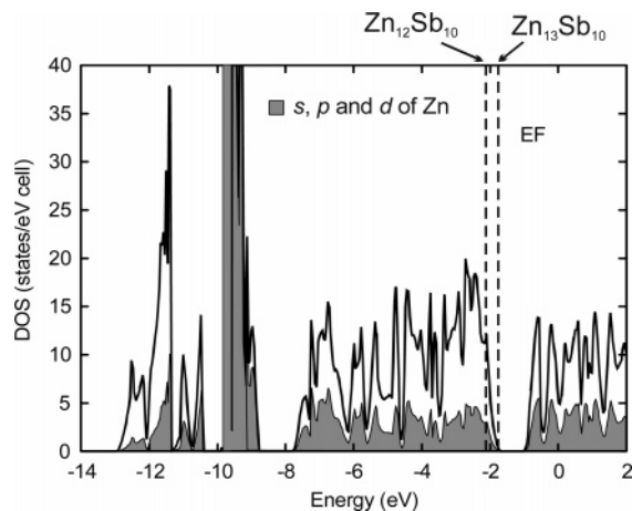
Figure 11. Total and partial DOS calculated assuming an idealized Zn_{12}Sb_{10} framework of \beta - Zn_{13}Sb_{10} . Dashed lines show positions of the Fermi level for the two compositions.
