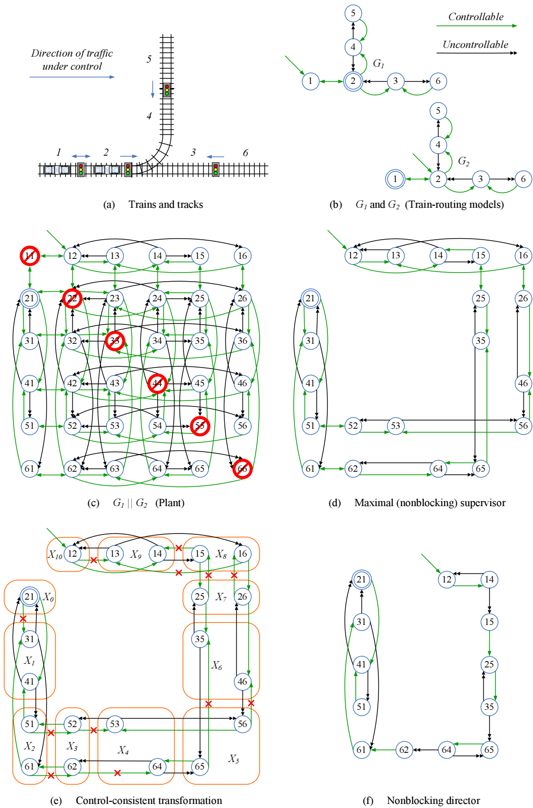
Figure 3.6 Synthesis of a nonblocking director for the application example
