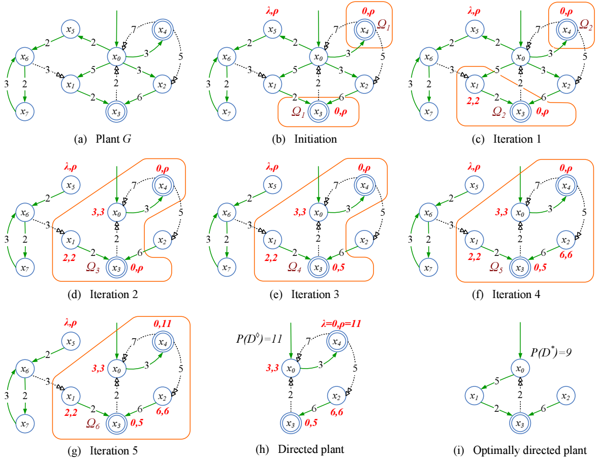
Figure 6.2 Example for Algorithm 8
