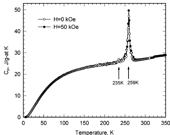
Figure 2. Heat capacity of the Zn_4Sb_3 sample measured from \sim 5 to 310 K in the 0 kOe magnetic field and from 80 to 350 K in the 50 kOe magnetic field. The arrows indicate the phase transitions at 235 and 259 K.
