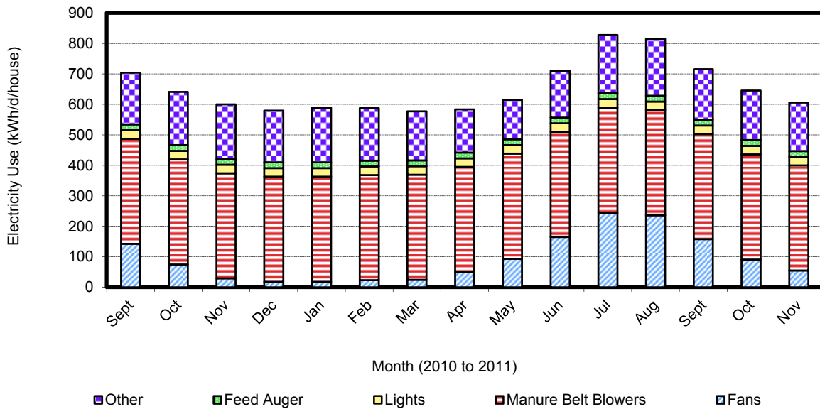
Figure 4. Monthly mean daily electricity use ( \text{kWh d}^{-1} ) partitioned into major components for the monitored aviary hen houses (~50,000 hens per house). Other components include egg belts, mixing fans, curtains on fans, and electrical outlets.
