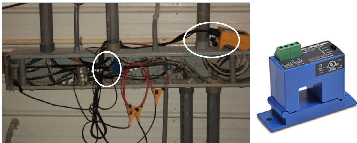
Figure 2. Left: the power logger (right oval) used to verify and develop power relationships for the inductive current sensors (left oval). The electric conduit cover was temporarily removed for making the measurement. Right: Close-up view of the current sensor.
