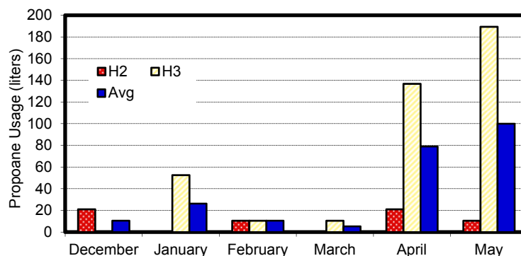
Figure 6. Monthly propane usage per barn of winter and spring 2010-2011.
