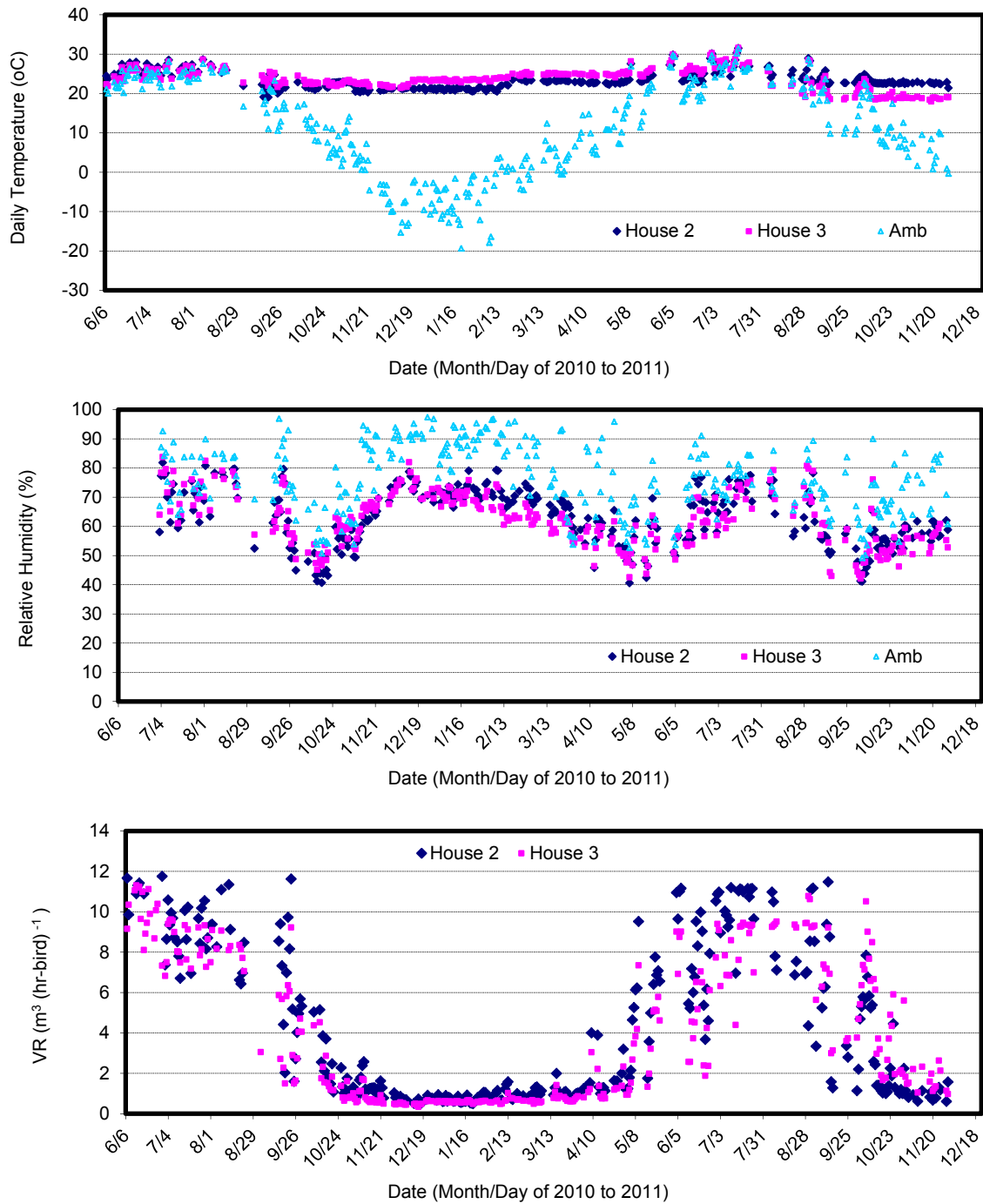
Figure 3. Daily temperature, relative humidity (RH), and ventilation rate (VR) of the two aviary houses monitored and the ambient (unit conversion: °F = 1.8×°C + 32; m³ h -1 = 0.589 CFM).
