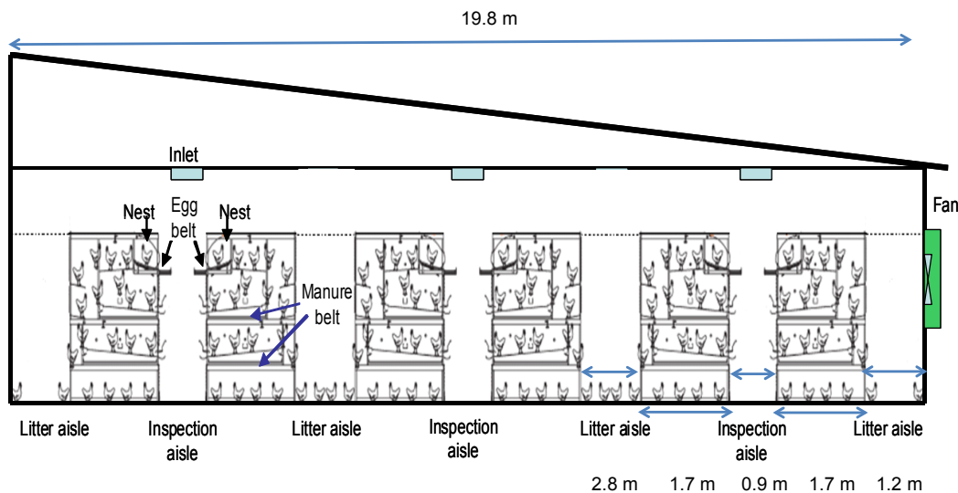
Figure 1. Cross-sectional view of the aviary hen house (one side of the double-wide house) monitored in this study (conversion: 1 m = 3.28 ft).
