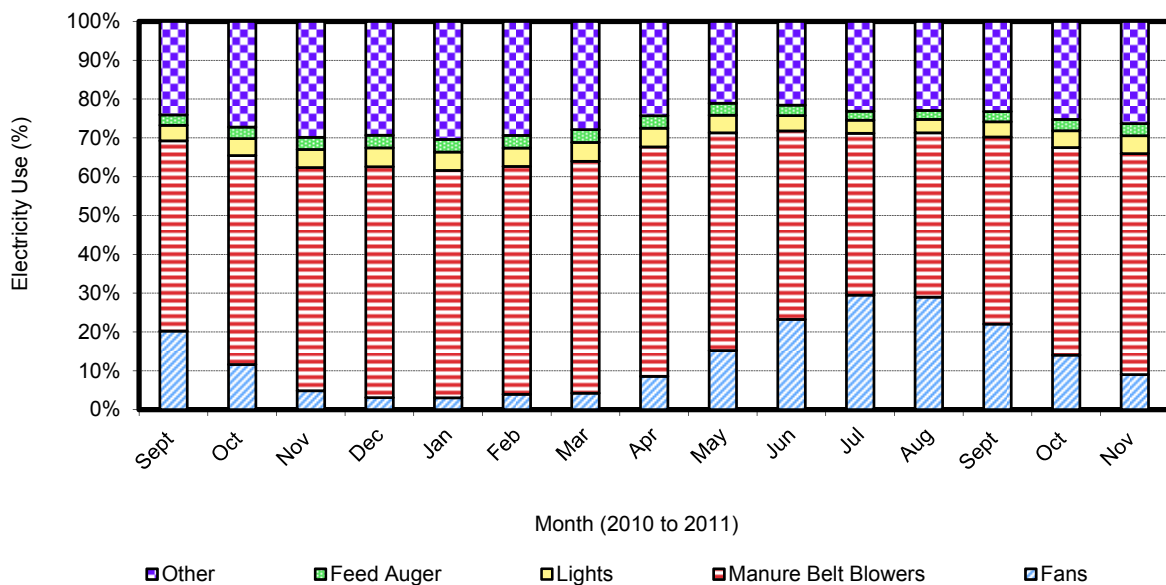
Figure 5. Electricity use distribution among major components (as % of monthly total) for the monitored aviary hen houses (~50,000 hens per house). Other components include egg belts, mixing fans, curtains on fans, and the electrical outlets.
