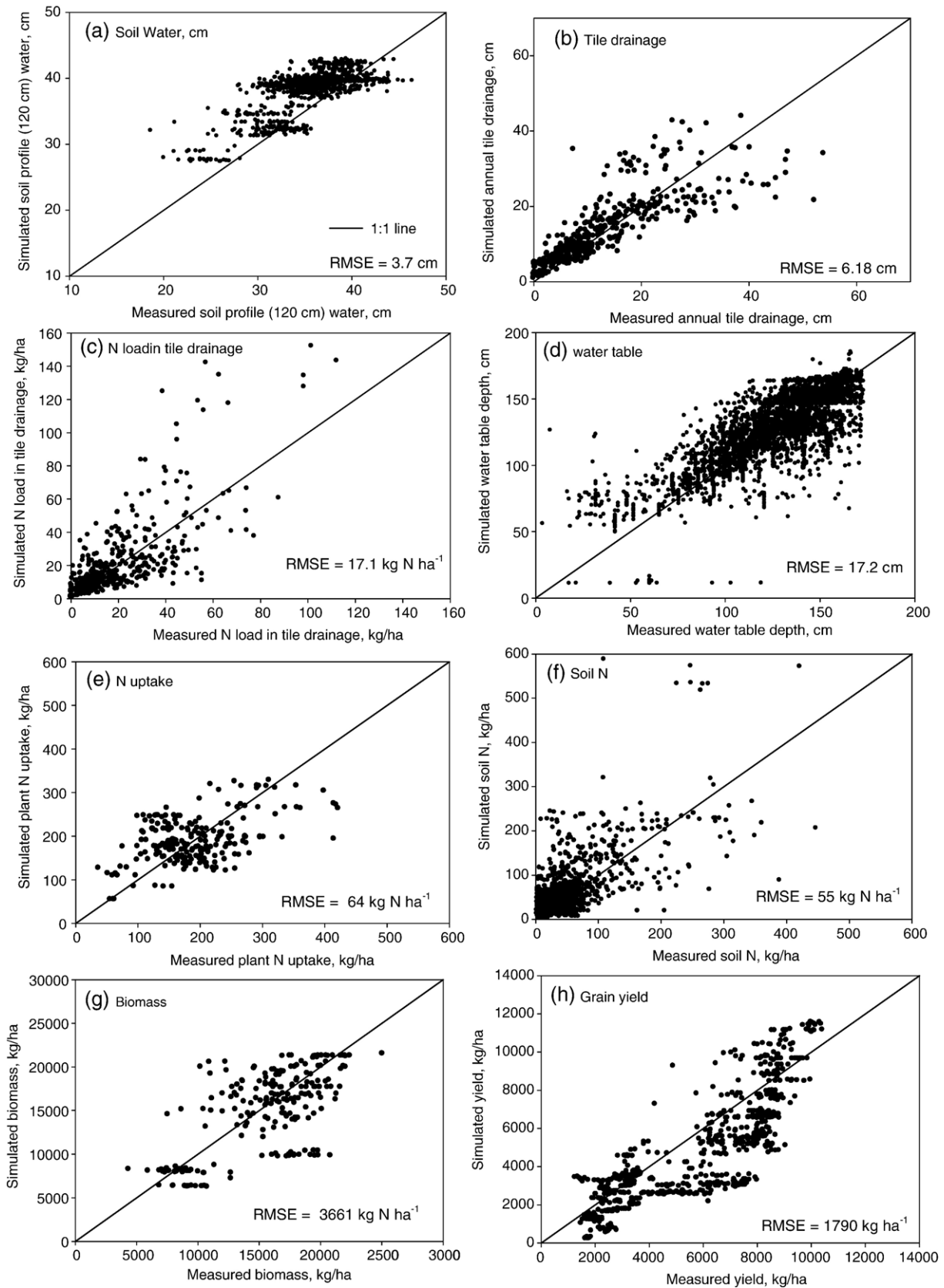
Fig. 2. Measured and simulated soil profile water, annual tile drainage, annual N load in tile drainage, water table depth, residual soil N, biomass N uptake, and grain and biomass yield for all the 30 plots (every plot and year are treated as a unique value) in the Nashua experiments.
