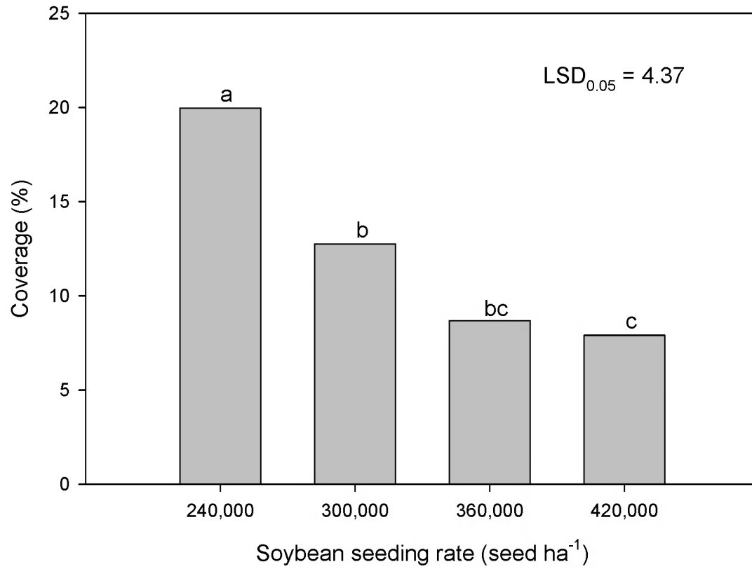
Figure 1. Spray coverage of water sensitive cards as influenced by the canopy of four soybean densities at V6 soybean stage.
