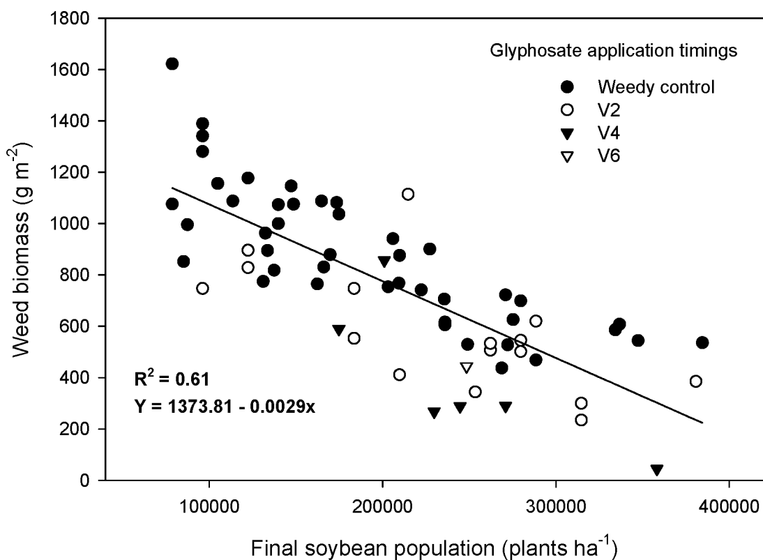
Figure 2. Relationship between final plant population and end-of-season weed biomass at Boone, Hancock, and Story, Iowa (2005–2006). Data were pooled across years, locations, herbicide application timing, and soybean densities and regressed against final plant population; where x = final soybean plant population ha -1 .
