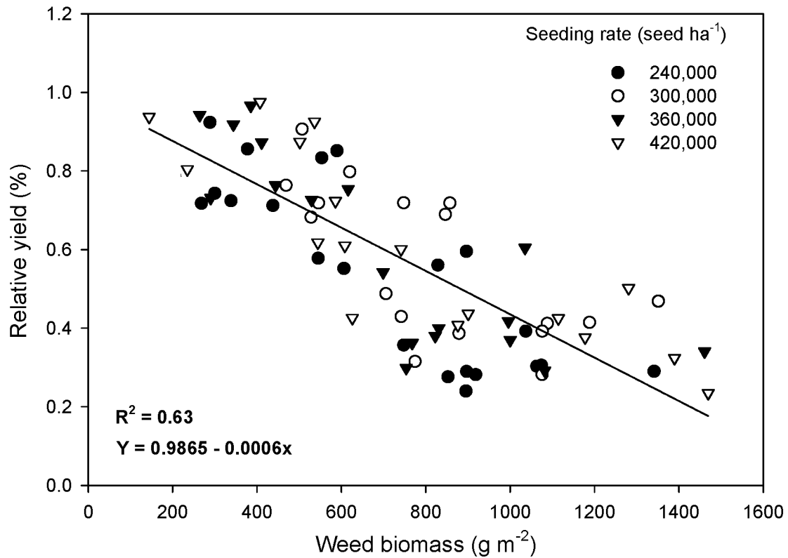
Figure 3. Relationship between weed biomass and soybean yield loss within four soybean seeding rates in Iowa (2005–2006). Data were pooled across year, location, herbicide application timing and regressed against weed biomass; where x = \text{g weed biomass m}^{-2} .
