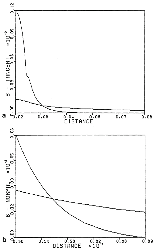
Figure 3. Flux density for a ferromagnetic tube ( r=50 ). a. Tangential component of flux density, b. Normal component of flux density.
