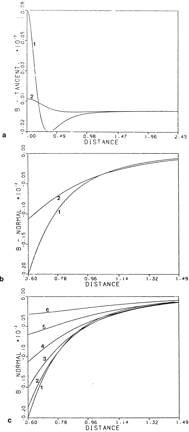
Figure 2. Flux density for coil in air. a. Tangential component of the flux density, b. Normal component of flux density, c. Normal component at six locations: r_1 > r_2 > r_3 > r_4 > r_5 > r_6 .
