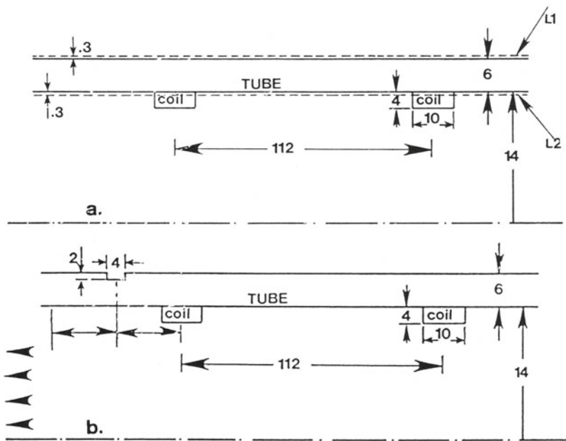
Figure 1. Geometry modeled. Dimensions are in mm. The two dotted lines show where comparisons are made. In lb, the coils are moving to the left.
