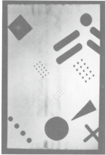
Fig. 10. Laminogram of copper/steel phantom; processing time was 10 minutes.
