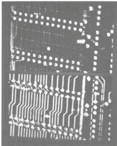
Fig. 7. Laminograms through plane 3, top, and plane 4, bottom.
