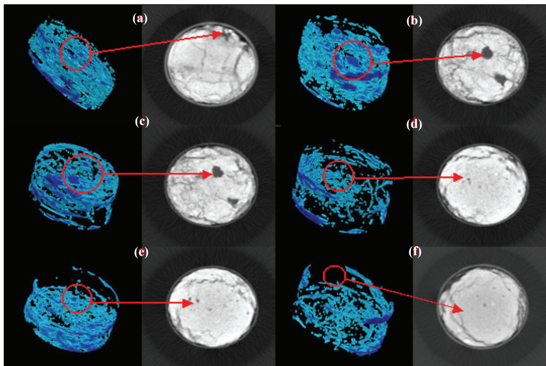
Figure 2. Macroporosity distribution in the top 15.3 cm soil profile for a chisel-plow (CP) tillage treatment using x-ray computed tomography (CT). Soil depth ranges of 0 to 5.1 cm, 5.1 to 10.2 cm, and 10.2 to 15.3 cm are depicted in images a-b, c-d, and e-f, respectively.
