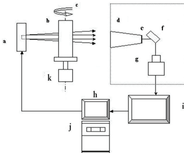
Figure 1. Schematic diagram of the x-ray CT scanner system: a = x-ray tube, b = fan beam, c = rotation axis, d = shutter and image intensifier, e = objective lens, f = mirror, g = camera, h = CPU, i = frame grabber, j = x-ray control panel, and k = platform positioner controller.
