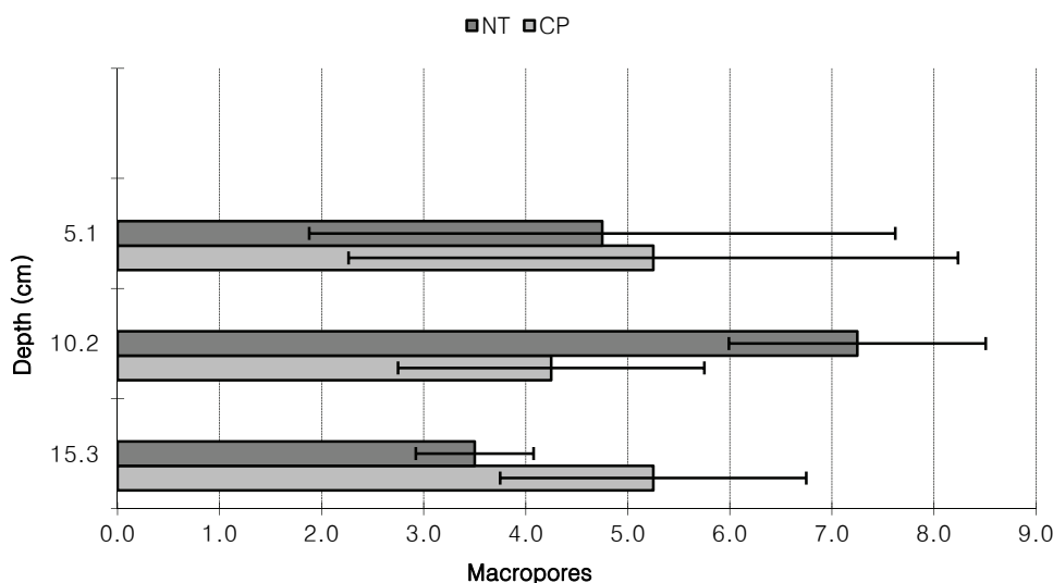
Figure 3. Average macropore number distribution as a function of three soil core sampling depths (5.1, 10.2, and 15.3 cm) and two soil tillage treatments, no-till (NT) and chisel-plow (CP), using x-ray computed tomography (CT). Error bars indicate \pm 1 standard deviation of the mean.
