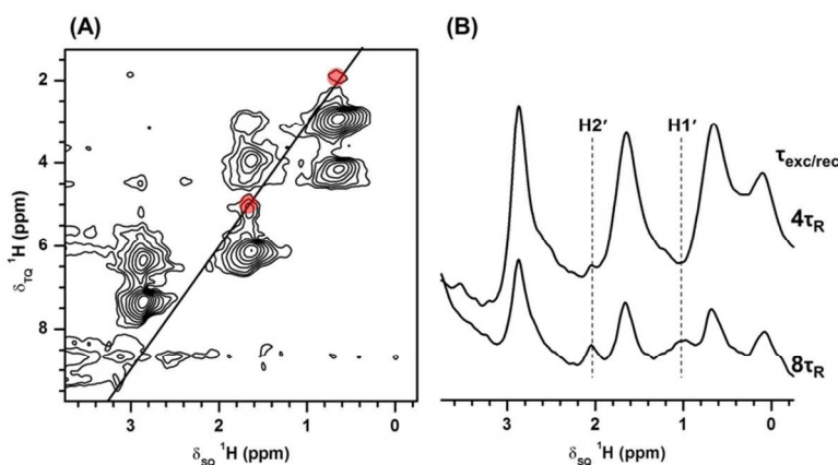
Figure 5. 2D 1 H TQ/SQ MAS and 1D TQ-filtered 1 H MAS spectra of AP-0.1. The spectra were obtained using \nu_{\text{R}} = 36 kHz, \nu_{\text{RF}}(^1\text{H}) = 100 kHz, \tau_{\text{z}} = 1 ms, \tau_{\text{RD}} = 2.0 s. The 2D 1 H TQ/SQ spectrum (A) was taken with \tau_{\text{exc/rec}} = 4\tau_{\text{R}} (111.1 \mu\text{s} ), 256 rows with \Delta t_1 = 27.778 \mu\text{s} , NS = 96, and AT = 27.3 h. The 1D TQ-filtered 1 H spectra (B) were collected using NS = 768.
