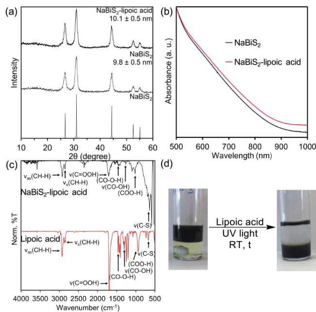
Figure 6. (a) Powder XRD, (b) solution-phase absorption spectra, and (c) IR spectra of NaBiS 2 nanocrystals before and after photochemical ligand exchange with lipoic acid. (d) Upon exchange, the nanocrystals transfer from the hexanes phase to methanol.
