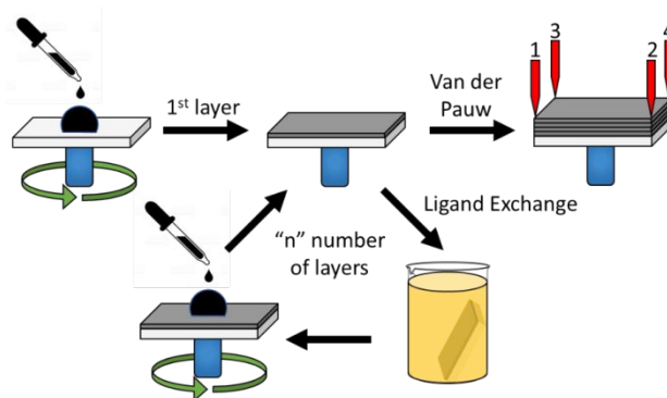
Scheme 3. Illustration of solid-liquid ligand exchange performed by the layer-by-layer (LbL) method.
