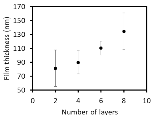
Figure 8. Film thickness of NaBiS 2 films as a function of layer-by-layer (LbL) NaI/NH 4 Ac-treating cycles. Standard deviation was determined by 3 measurements using a proflorimeter.
