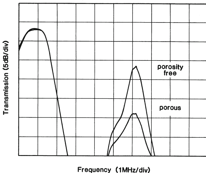
Fig. 4. Transmission spectra through porosity-free and porous parts of a composite plate (sample #ACL 6804).
