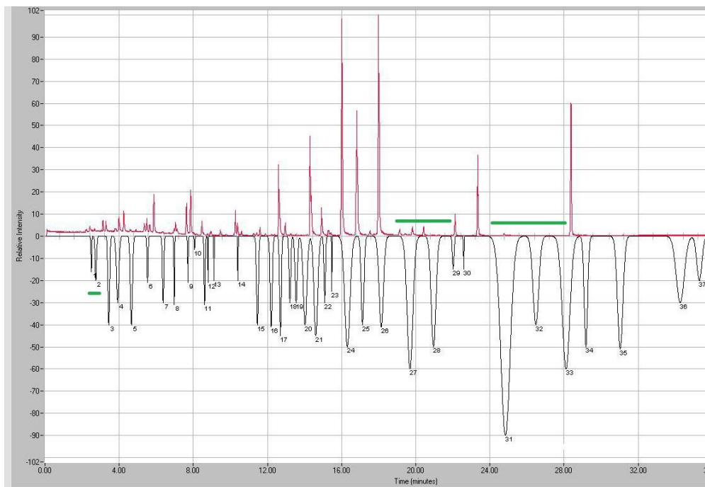
Figure 3. An overlay of aromagram and total ion chromatogram of the fresh cat feces exposed to SPME fiber for 50 min at 37 °C. An increase in black color signal height represents an increased intensity of odor, and the chromatogram is in the red color TIC signal. The green zone is showing that trace level concentration of malodors can produce an intense olfactory response detected by the panelist using GC-MS-O.
