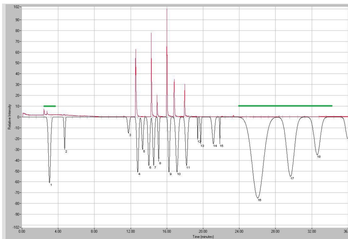
Figure 4: An overlay of aromagram and total ion chromatogram of the stale cat feces, equilibrated for 24 h and exposed to SPME fiber for 50 min at 37 °C. An increase in black color signal height represents an increased intensity of odor, and the chromatogram is in the red color TIC signal. The green zone is showing that trace level concentration of malodors can produce an intense olfactory response detected by the panelist using GC-MS-O.
