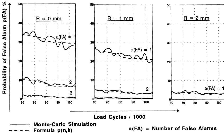
Figure 4. Validation of NDI "Monte-Carlo Simulation". Probability of false alarms p(FA) for various POD threshold levels R.
