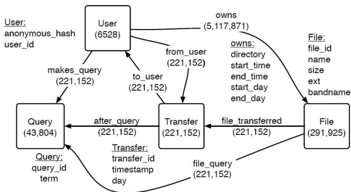
Figure 3.1 Data set
