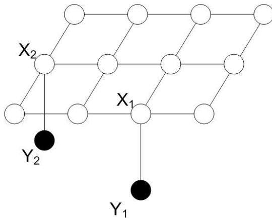
Figure 2.1 HMM model
