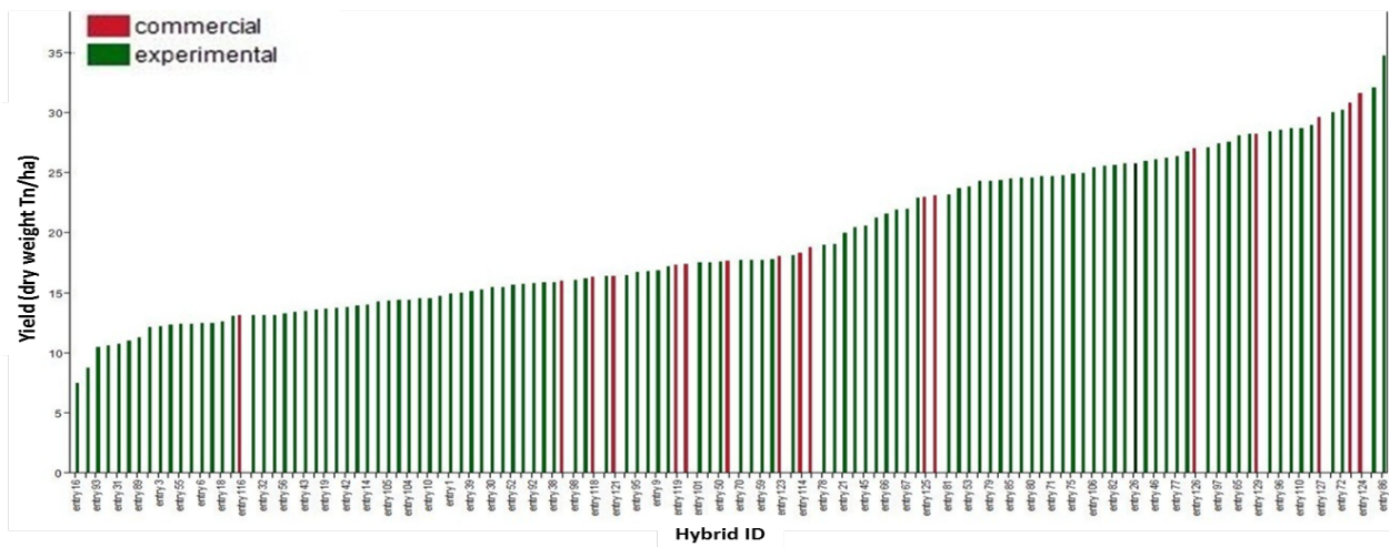
Figure 2. Biomass yield of experimental and commercial sorghum hybrids. Yields are averaged over replications and locations.
