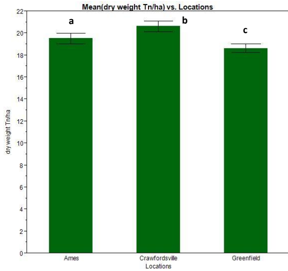
Figure 1. Average biomass yield per location. Each error bar represents one standard error from the mean. Locations not labeled with the same letter are significantly different at P \leq 0.05 (Tukey-Kramer test).
