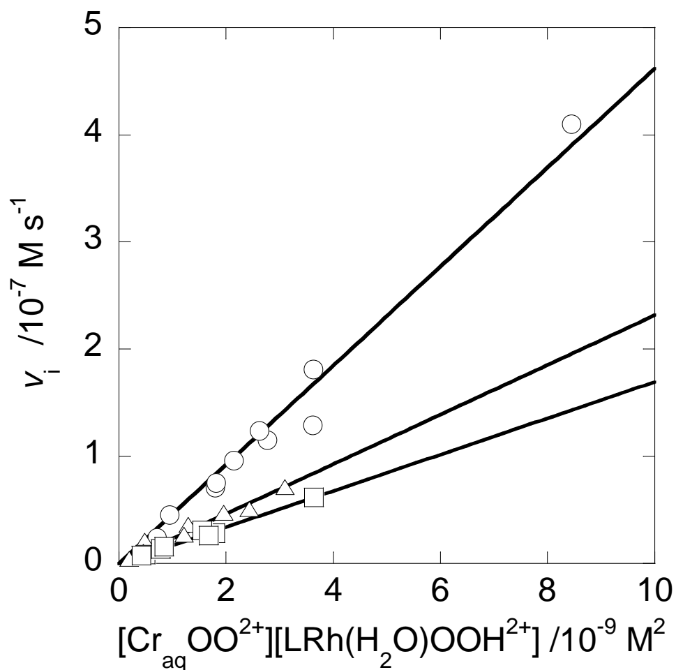
Figure 3. Initial rate as a function of ([\text{Cr}_{\text{aq}}\text{OO}^{2+}] \times [\text{LRh}(\text{H}_2\text{O})\text{OOH}^{2+}]) at 25 °C. Slope = k = 46 \pm 2 \text{ L} = (\text{NH}_3)_4 = \text{O} , 23 \pm 1 \text{ L} = \text{L}^1 = \Delta , 17 \pm 1 \text{ M}^{-1} \text{ s}^{-1} \text{ L} = \text{L}^2 = \square .
