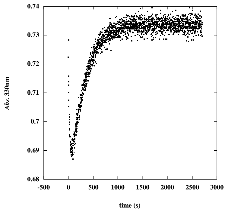
Figure. 4 Reaction of 4-piccoline-N-oxide as substrate with an extreme exogenous pyridine nucleophile excess. Conditions: [1] = 2 \times 10^{-5} \text{ mol L}^{-1} ; [\text{PPh}_3] = 2.5 \times 10^{-2} \text{ mol L}^{-1} ; [\text{pyridine}] = 4.9 \text{ mol L}^{-1} ; [\text{picO}] = 2 \times 10^{-4} \text{ mol L}^{-1} .
