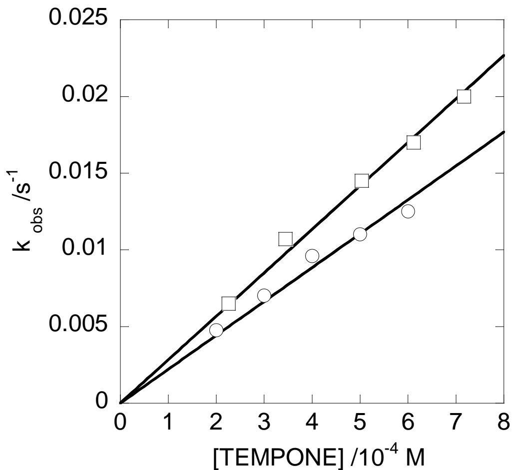
Figure 3. k_{\text{obs}} vs. [\text{TEMPONE}] concentration for the reaction of \text{Cr}_{\text{aq}}\text{OO}^{2+} with TEMPONE at 25 °C. Conditions: \circ in 0.02 M \text{HClO}_4 ; \square in 0.10 M \text{HClO}_4 ; [\text{Cr}_{\text{aq}}\text{OO}^{2+}] = 3.4 - 9.0 \times 10^{-5} \text{ M} ; Slope = k = 28 \pm 0.5 \text{ M}^{-1} \text{ s}^{-1} for \square ; 22 \pm 0.6 \text{ M}^{-1} \text{ s}^{-1} for \circ ; \mu = 0.1 \text{ M} ( \text{NaClO}_4 balance).
