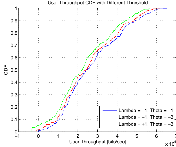
Figure 6.3 User Throughput CDF with Different (\lambda, \theta) , Transmission Mode 4
