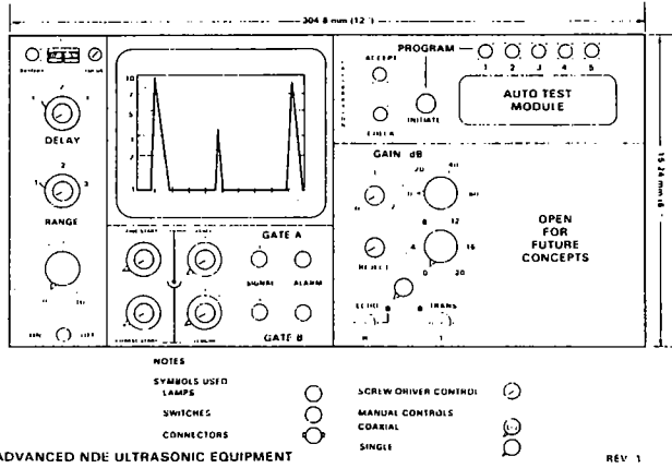
Figure 1. Concept of Advanced Ultrasonic System Control Panel
