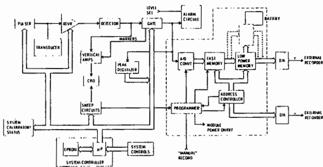
Figure 4. Advanced Ultrasonic Equipment - Breadboard Concept
