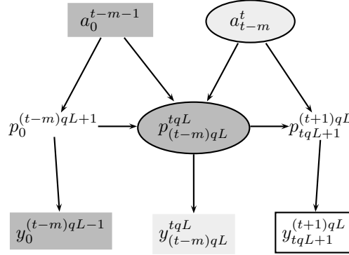
Figure 3.2: Dependence path.
