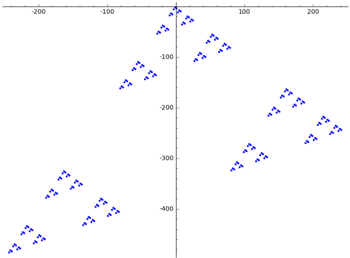
Figure 4.7 Plot of s_5(-1, -2) .
