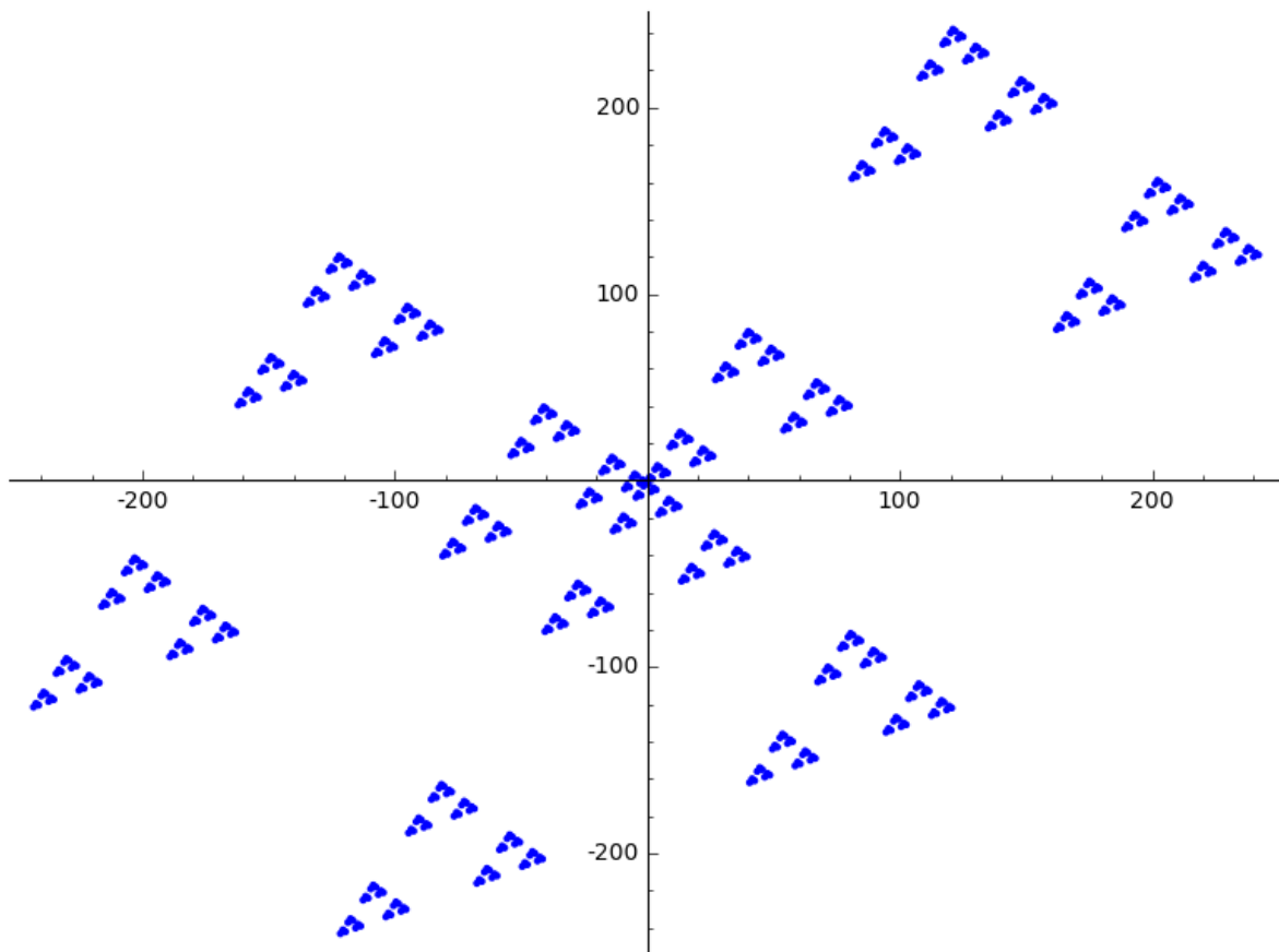
Figure 4.4 Plot of r_5(0,0) \cup r_5(-1/2, -1) \cup r_5(-1, -1/2) .
