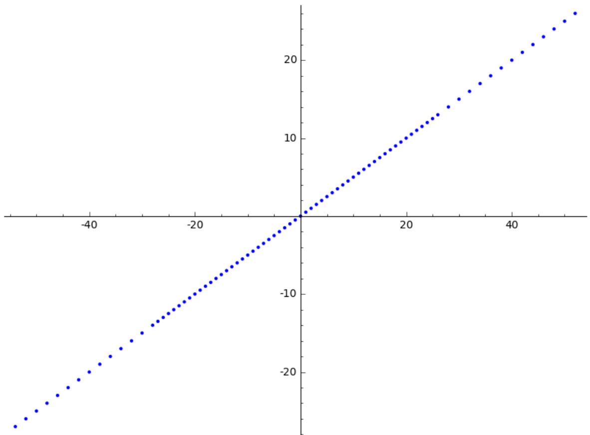
Figure 4.3 Plot of l_3(0,0) \cup l_3(-1,-1/2) \cup l_3(-2,-1) .
