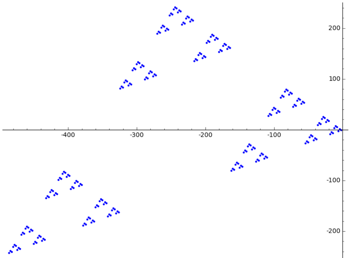
Figure 4.8 Plot of s_5(-2, -1) .
