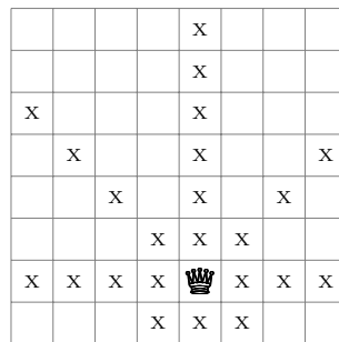
Figure 1.2 Potential moves of a queen chess piece
