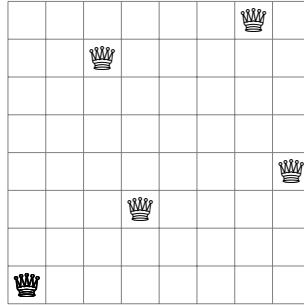
Figure 1.3 Solution to the Five Queens Problem
