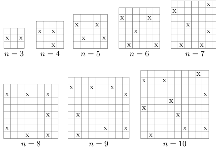
Figure 2.5 Minimum exponential dominating sets of \mathcal{S}_n , 3 \leq n \leq 10 .
