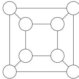
Figure 1.4 Hypercube Q_3 .
