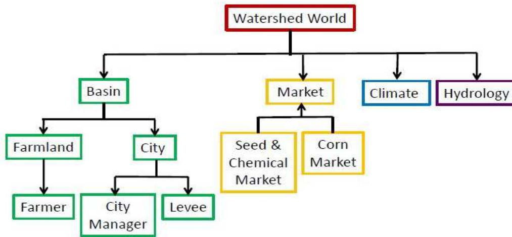
Figure 2: Agent taxonomy for an ACE watershed model. Up-pointing arrows denote “is a” relationships and down-pointing arrows denote “has a” relationships. Source: Tesfatsion et al. (2017).
