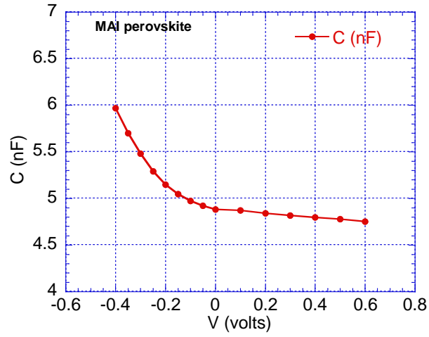
Supplementary FIG. 1. Capacitance-voltage measurements for the MAI (glass/ITO/NiO/MAI PVSK/PCBM60/Al) perovskite device.
