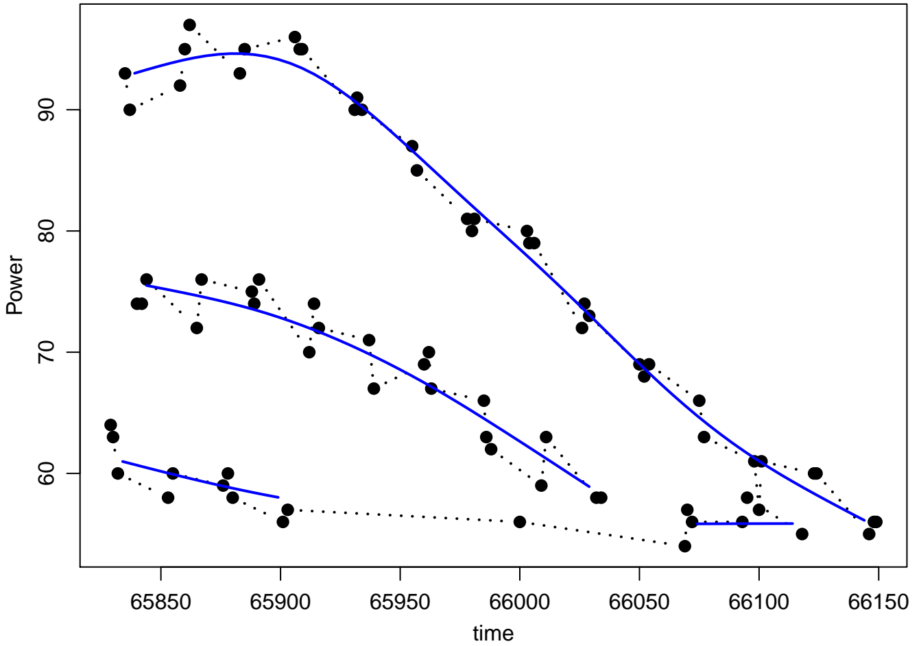
Figure S5: Using thin-plate regression smoothing provided an effective alternative to calculating the median power recorded over time. Dots and dashed lines show observed power readings readings for three antennae on one tower over time, colored lines show smoothed values. The effective degrees of freedom are 1.8, 2.0, and 4.6.
