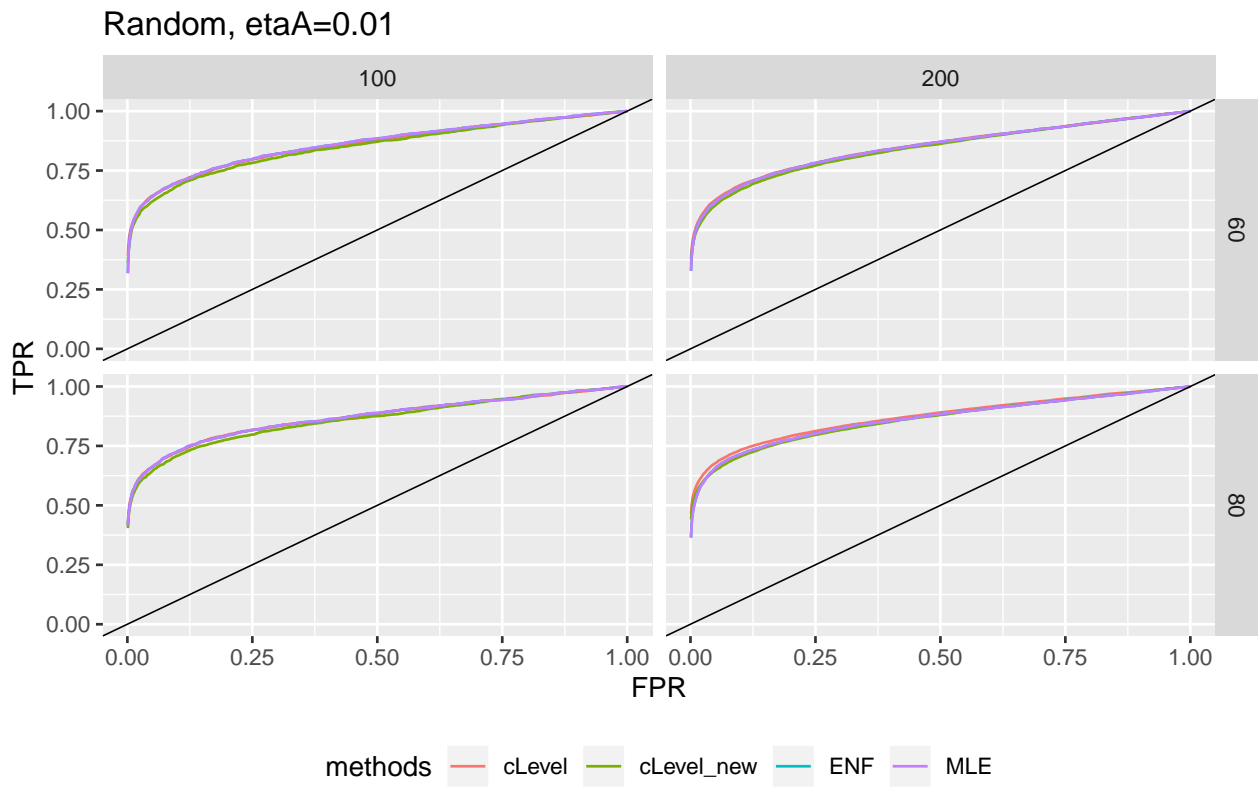
Figure 1: ROC curve, Random 0.01
