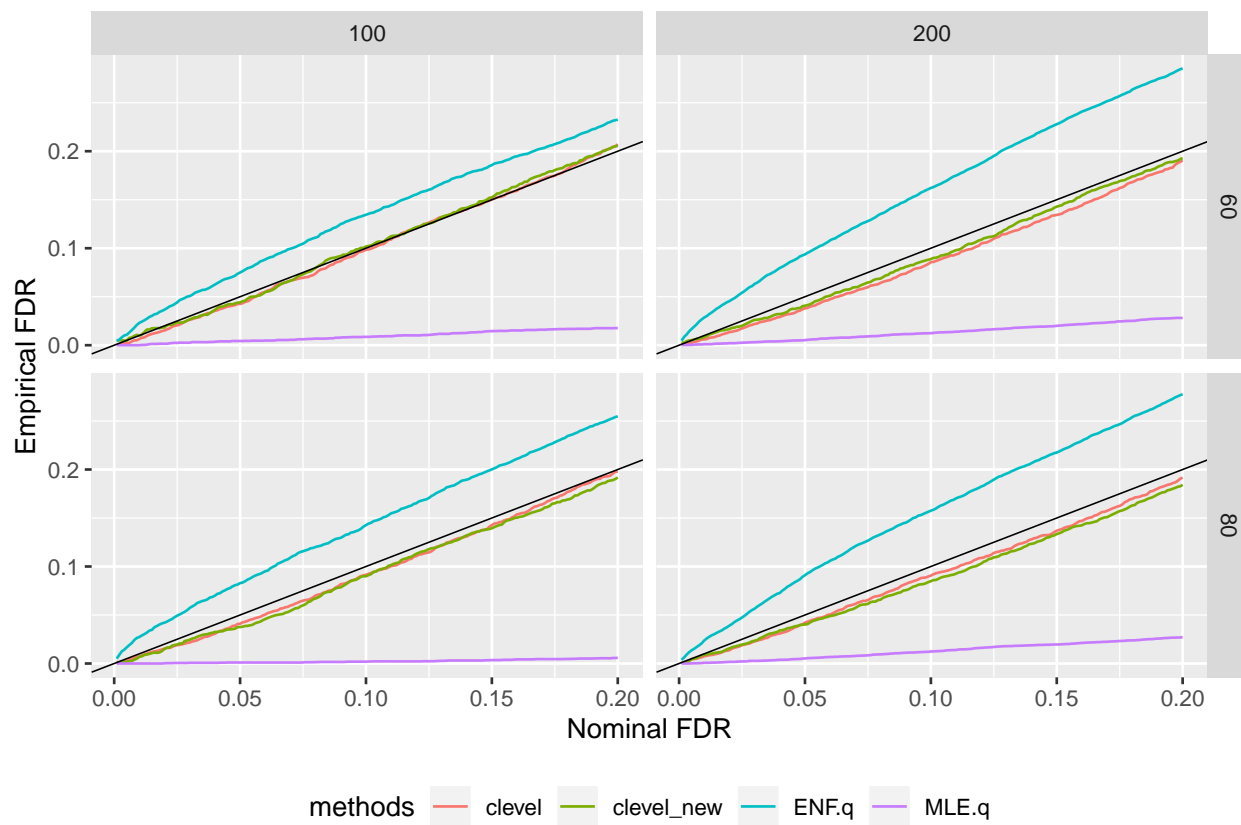
Figure 6: fdr, BD 4 by 4
