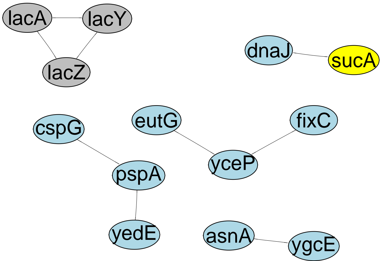
Figure 10: Network by Shrunk MLE (adjusted)
