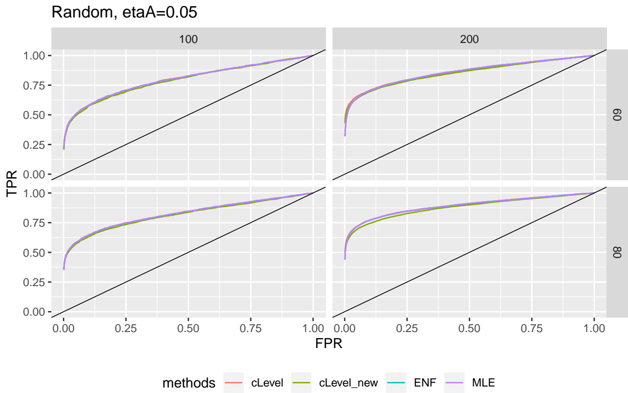
Figure 3: ROC curve, Random 0.05
