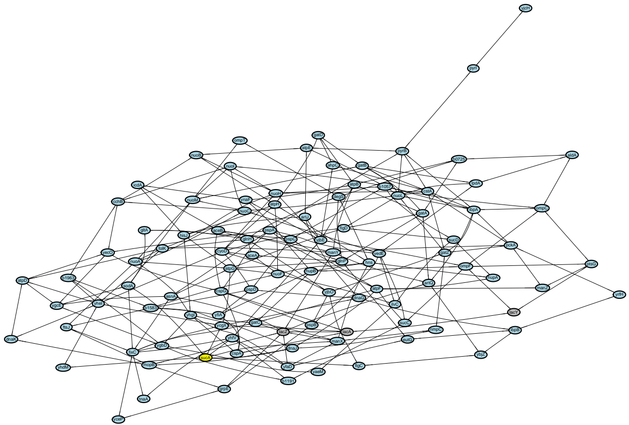
Figure 8: Network by 0-PCG (cv)
