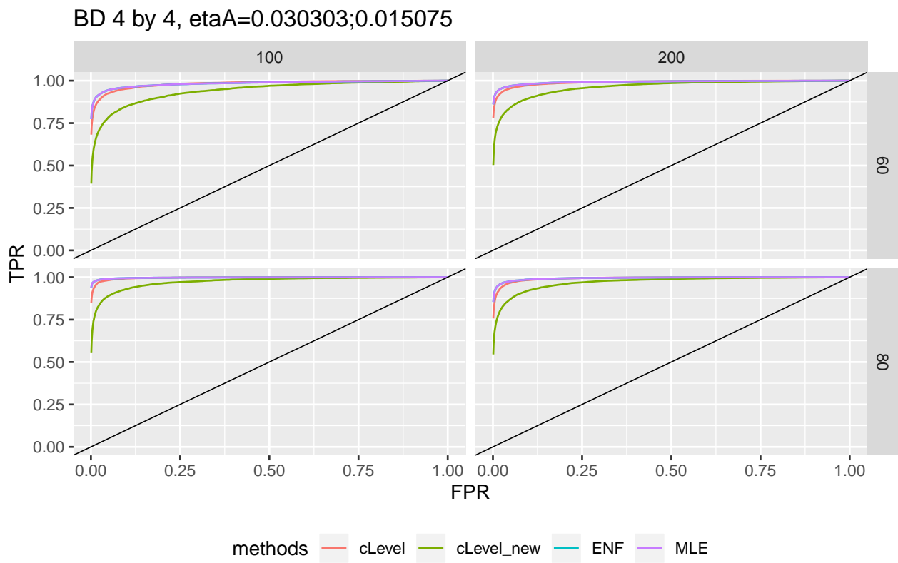
Figure 5: ROC curve, BD 4 by 4
