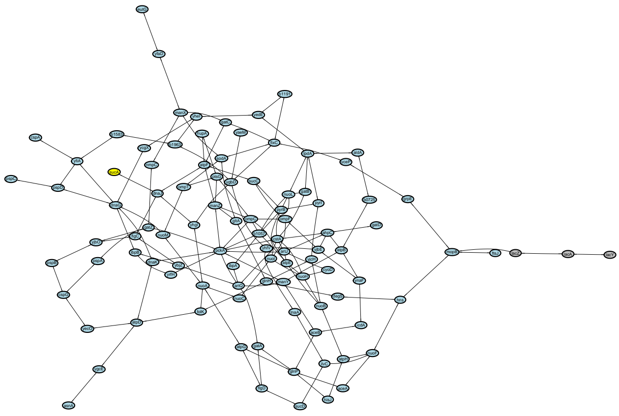
Figure 9: Network by 0-PCG (df=7)
