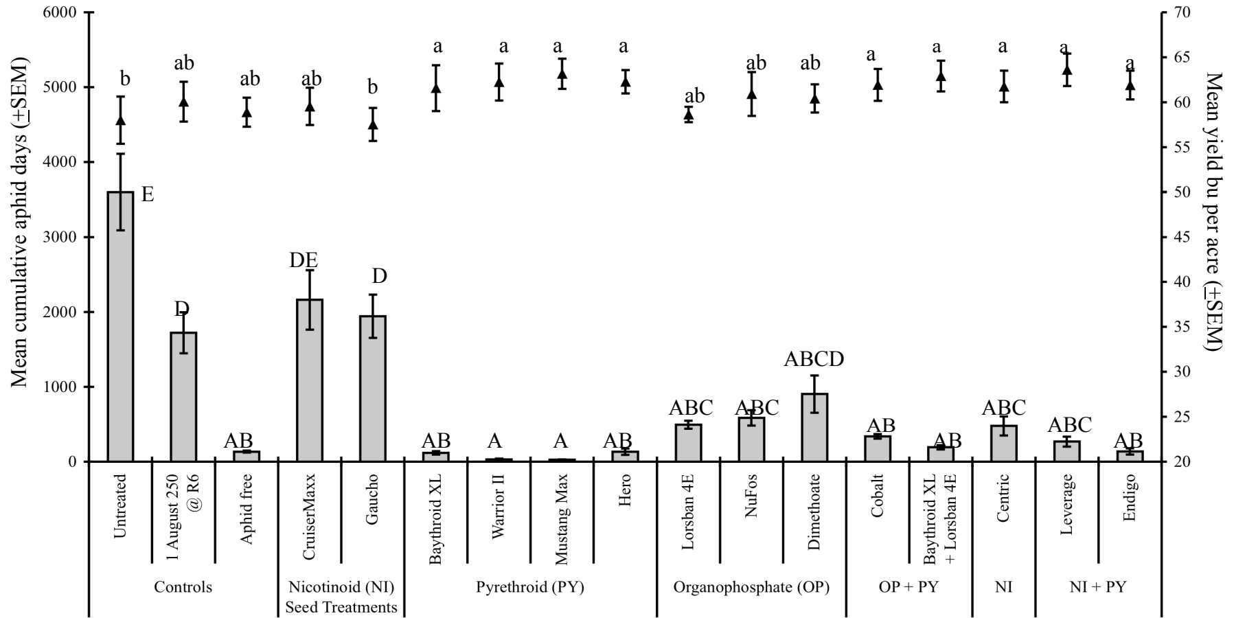
Figure 1. Impact of insecticides aphid exposure and yield in 2008. Soybeans were planted on May 15 and insecticides were applied prior to planting to selected plots. The aphid free control was treated with insecticides three times (July 22, August 1, and August 22), all other foliar applied insecticides were applied on August 1. Cumulative aphid days are represented by bars and capital letters. Yields are represented by triangles and lowercase letters. Means with a unique letter are statistically different ( P \leq 0.05 ).
